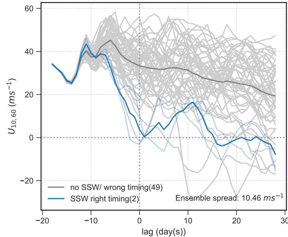
(c) ECMWF real-time forecast 2018-01-29
