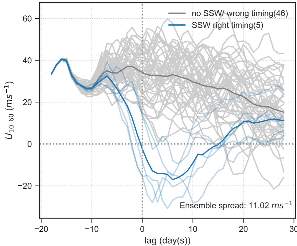
(a) ECMWF real-time forecast 2018-01-25
