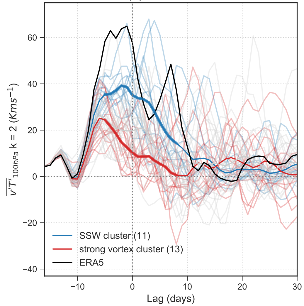
(c) \overline{v'T'} k = 2
