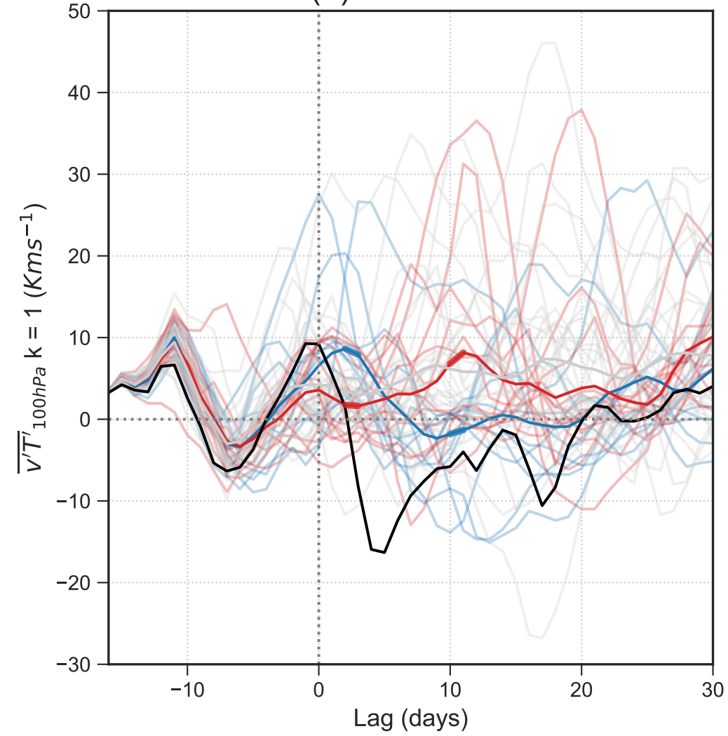
(b) \overline{v'T'} k = 1
