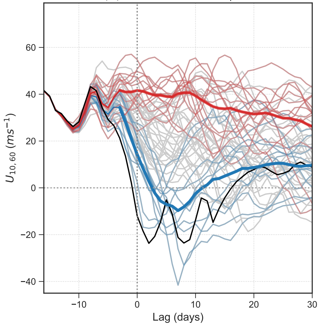
(a) 2018 SSW: U_{10,60}
