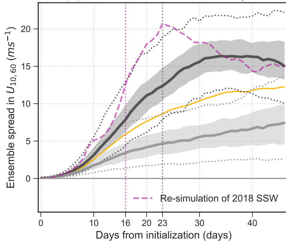
(a) Ensemble spread in U_{10,60}
