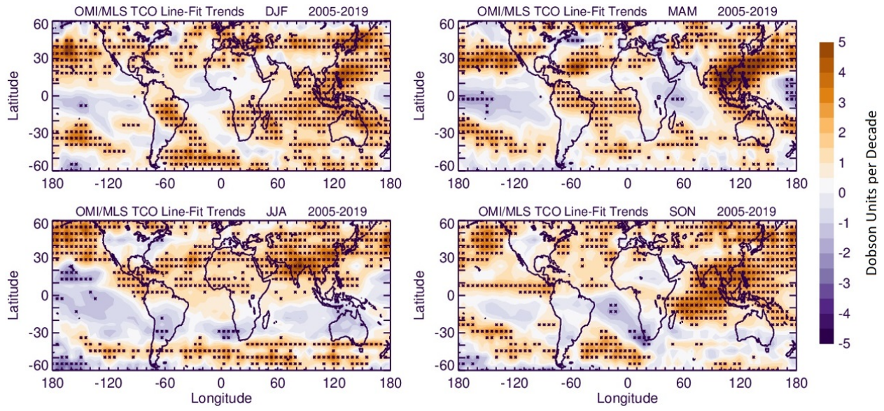
Figure S 7: Seasonal trends in tropospheric column ozone from 2005 to 2019. Asterisks denote 95% confidence trends.
