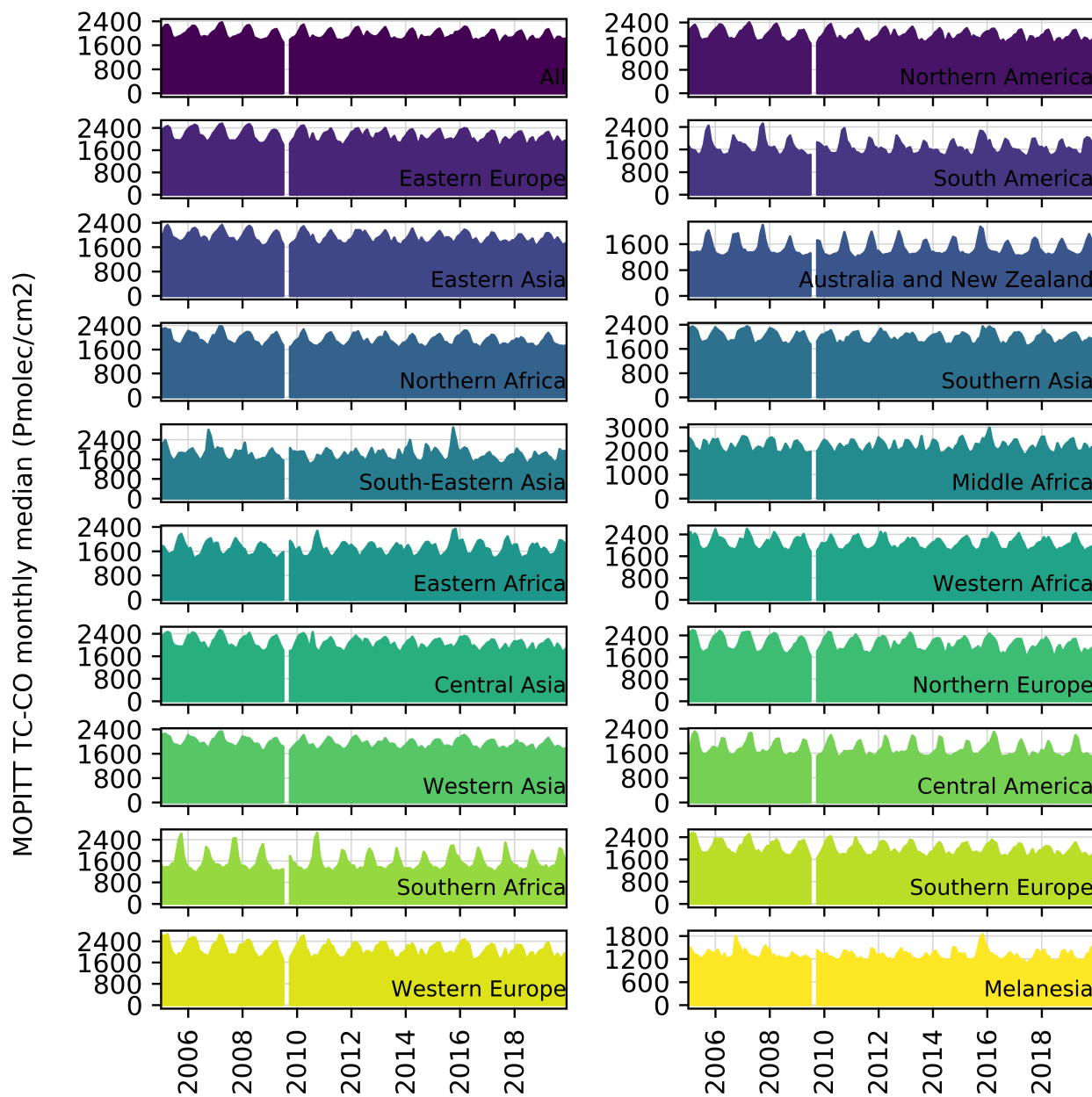
Figure S 4: Monthly regional time series of MOPITT TC-CO.
