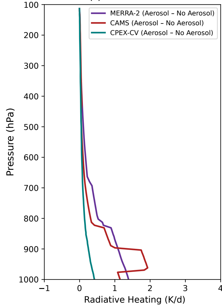
(c) TOTAL HEATING
