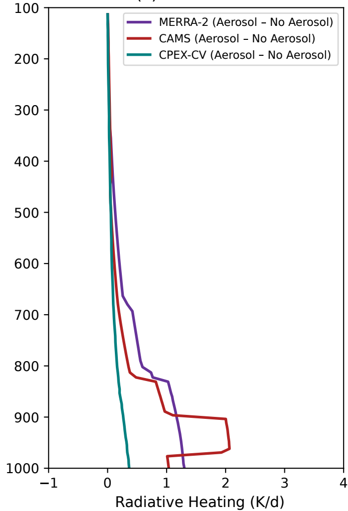
(a) SW HEATING
