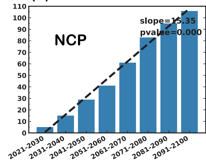
(c) SSP126
