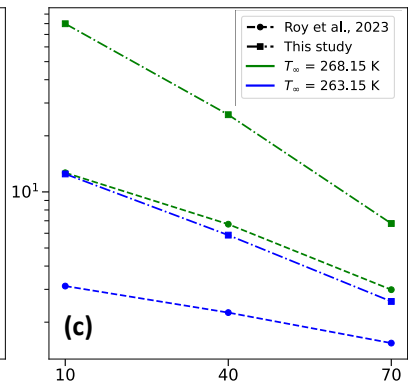
(iii) Demott Scheme ( N_a = 0.1 per cc)
