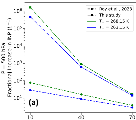
(i) Fletcher Scheme
