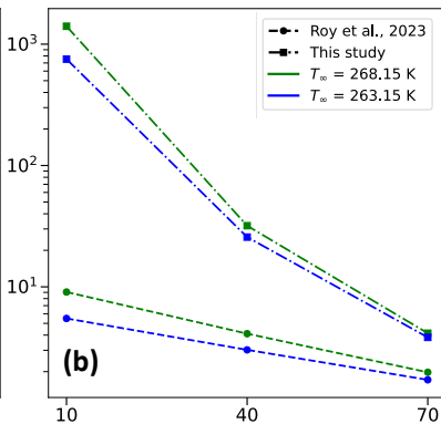
(ii) Cooper Scheme
