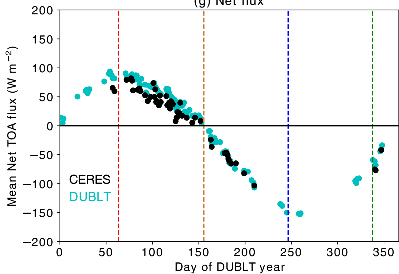
(g) Net flux
