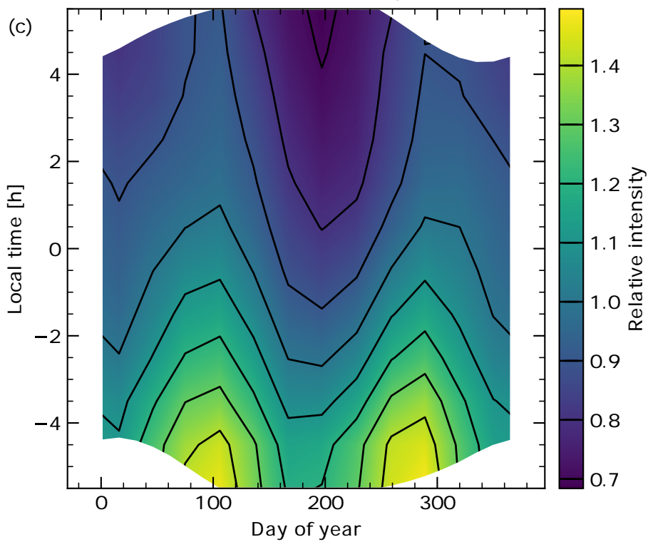
HO 2 emission from H + O 3 (R14)
