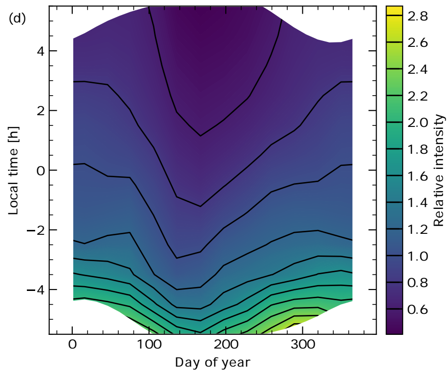
HO 2 emission from R8 + R9 + R14
