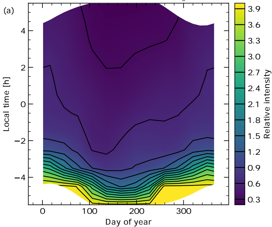
HO 2 emission from H + O 3 (R14)
