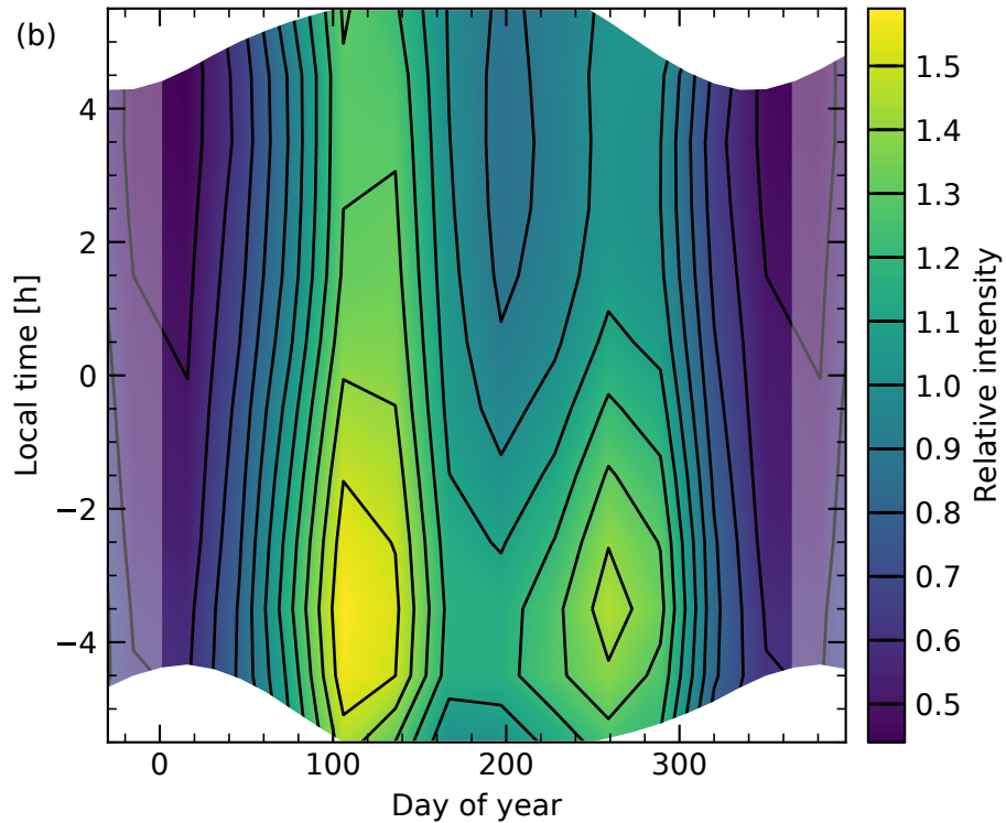
OFeOH emission from FeOH + O 3 (R6)
