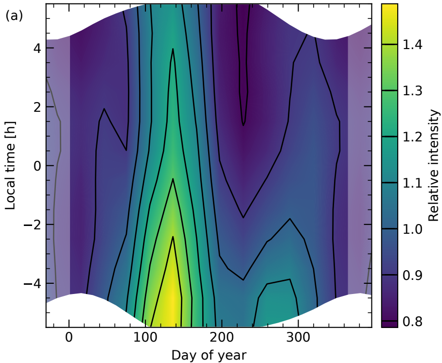
FeO emission from Fe + O 3 (R2)
