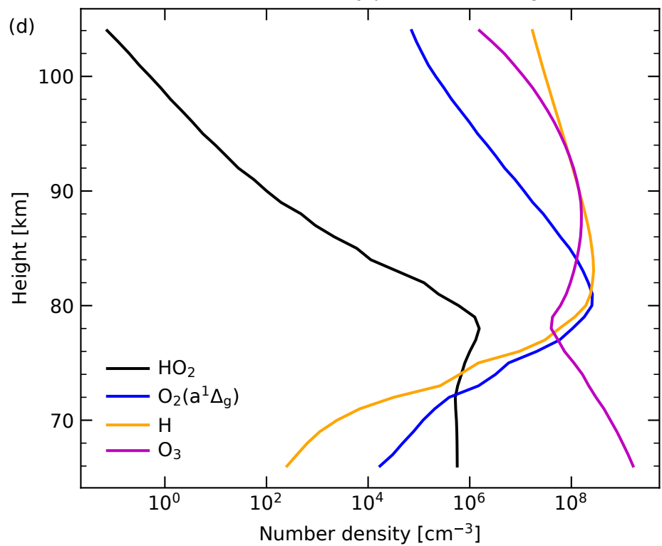
HO 2 -related density profiles at midnight
