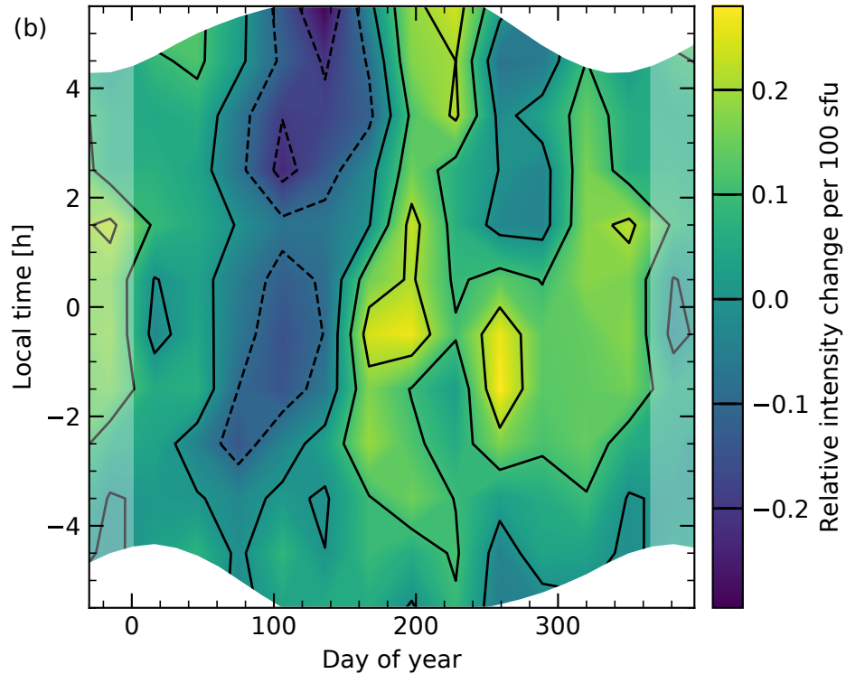
Feature at 1510 nm indicating X
