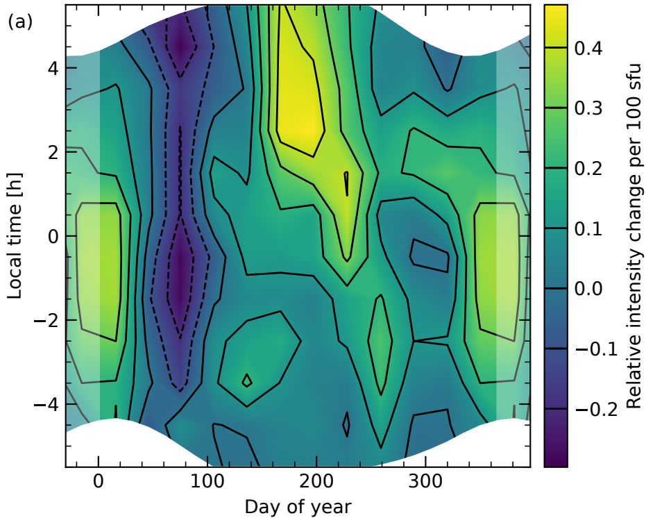
Feature at 595 nm indicating FeO
