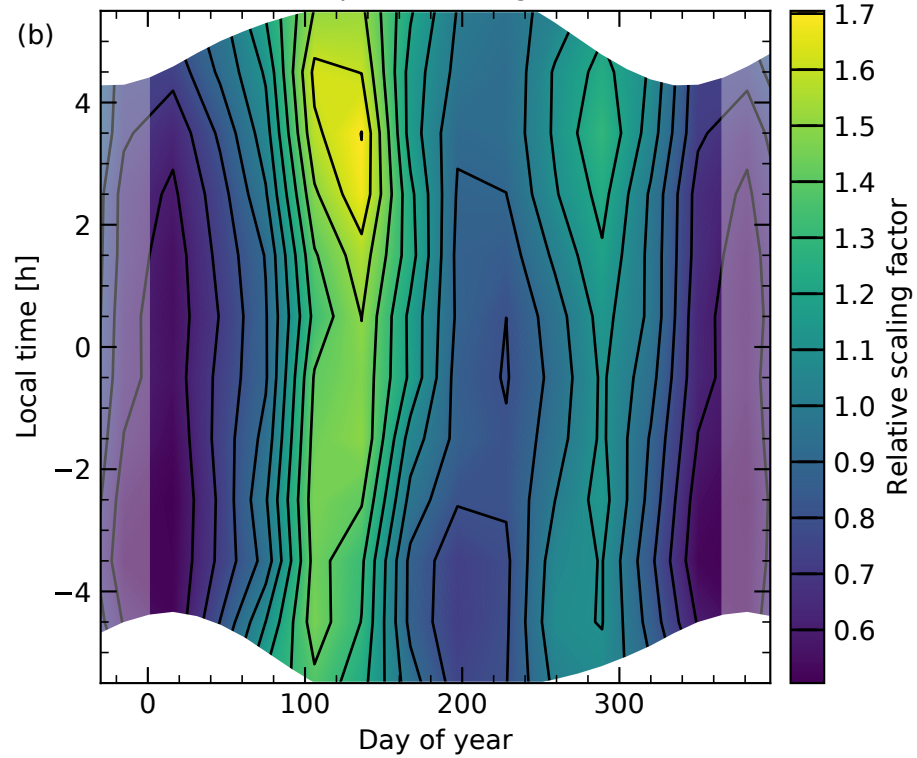
NMF comp. 4 indicating O 2 (UVB)
