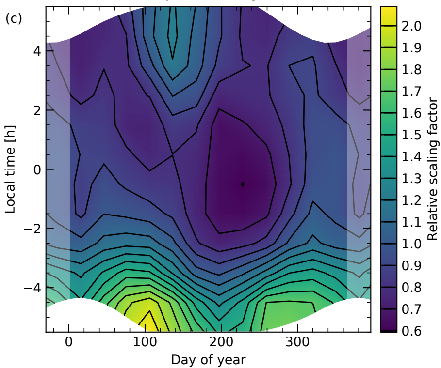
NMF comp. 3 indicating O 2 (NIR)
