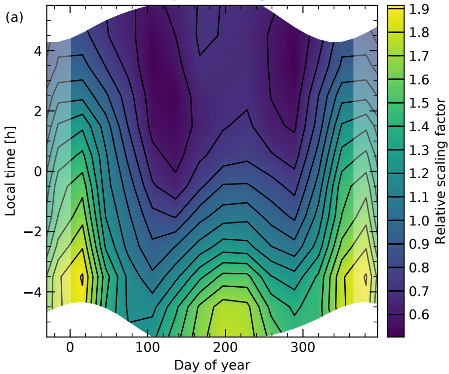
NMF comp. 3 indicating O 2 (NIR)
