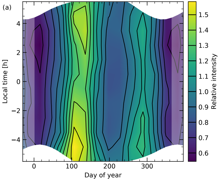
Feature at 595 nm indicating FeO
