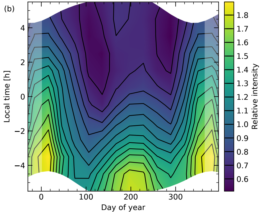
Feature at 1510 nm indicating X
