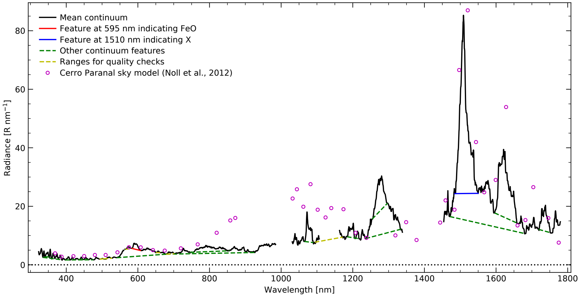
Mean X-shooter-based nightglow continuum
