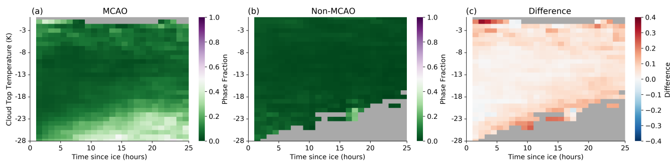
Figure S1. Evolution of ice phase fraction as a function of time and cloud top temperature for (a) MCAO, (b) non-MCAO. (c) is the difference between them. Grid points with fewer than 500 successful retrievals are coloured in grey.
