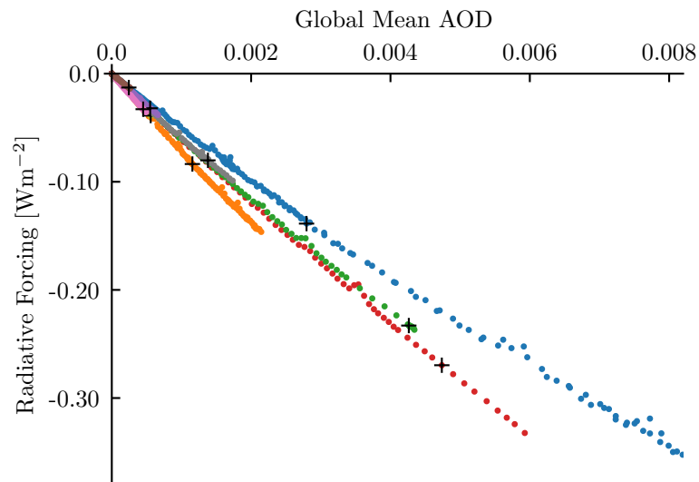
(b) Clear-sky Aerosol Forcing with Equal SSA
