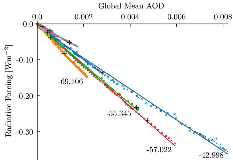
(a) Clear-sky Aerosol Forcing
