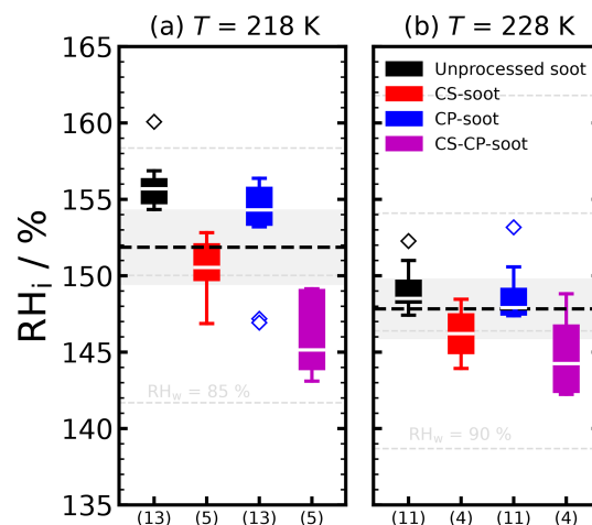
Figure 2. Ice nucleation onset \text{RH}_i range ( \text{AF} = 10^{-3} ) of unprocessed and processed soot at the given temperatures. The boxes extend from the 25th to 75th percentiles, the white bar shows the median, the whiskers include the inter-quartile range and the scatter points show the outlier data points. Panels (a) and (b) share the same y axis and legend. The dashed black line indicates \text{RH}_{\text{hom}} (Koop et al., 2000) and the grey shading its uncertainties in the HINC. The \text{RH}_w values are shown by the dashed grey lines in steps of 5 %. The x axis shows the number of measurements conducted per sample type (including different engine types).
