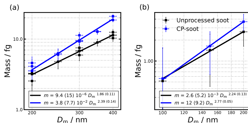
Figure 3. Unprocessed and contrail-processed size-selected aggregate mass mode ( m ) as a function of its electric mobility diameter ( D_m ) for (a) the CFM56-7B26/3, CFM56-5B4/P, CFM56-7B27/3 and CFM56-7B24/3 engines and (b) the PW4168A engine. Lines show fits to Eq. (2) with retrieved parameters shown in the boxes. Uncertainties in the parameters are shown in parentheses. Panel (b) shares its legend with panel (a).
