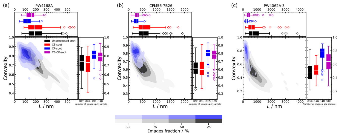
Figure 5. Maximum 2D-projected length ( L ) and convexity of unprocessed and processed aviation soot aggregates analyzed from TEM images for three engines. Convexity and L distributions are shown for all soot populations in the boxplots (box statistics are as in Fig. 2) and the density contours in the larger plots only for unprocessed and CP-soot for clarity. The colored areas enclose – from dark to light – about 25 %, 50 %, 75 % and 95 % of the images (one aggregate per image). The number of images analyzed is shown on the x axis below the boxplots. Panel (a) shares its legend with panels (b) and (c).
