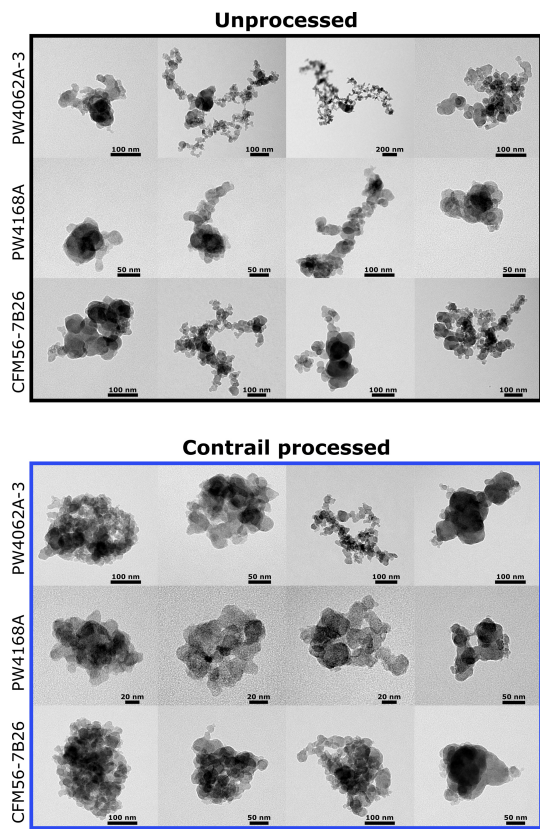
Figure A2. TEM images of unprocessed and contrail-processed soot aggregates for the given engines. Note the different scale bars in the images.
