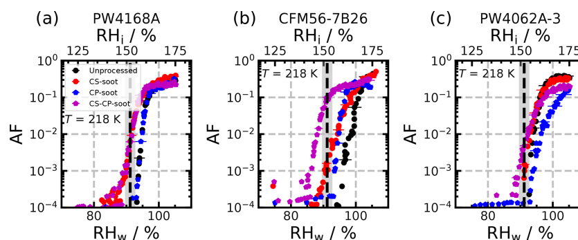
Figure 6. AF ice nucleation curves as a function of RH at 218 K for the given engines. The dashed black line and grey shading indicate RH_{\text{hom}} and associated uncertainties. Panel (a) shares its legend with panels (b) and (c).
