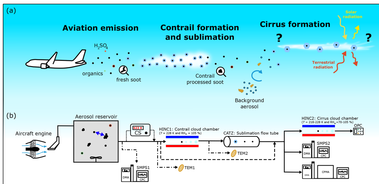
Figure 1. (a) Schematic of the main atmospheric processes associated with aviation soot–cirrus interaction. From left to right: due to the incomplete combustion of aviation fuel, aircraft engines emit soot particles externally and internally mixed with SO 2 / H 2 SO 4 and organics (unburned hydrocarbons, oil droplets). Plume particles (mainly soot and H 2 SO 4 ) can activate as cloud droplets and ice crystals (Kärcher, 2018; Voigt et al., 2021), forming a contrail cloud due to the high concentration of water vapor and low temperature that can immediately sublime or persist and subsequently sublime. The soot ice residuals released upon sublimation are referred to as contrail-processed soot particles. Background aerosol (e.g., dust, solution droplets) and soot can both nucleate ice and form in situ cirrus clouds. (b) Experimental setup mimicking the aviation soot atmospheric processes shown in (a). Arrows show the direction of the aerosol flow. See text for details. Abbreviations: CS, catalytic stripper; SMPS, scanning mobility particle sizer; DMA, differential mobility analyzer; CPC, condensation particle counter; HINC, horizontal ice nucleation chamber; TEM, transmission electron microscopy; CATZ, cloud aerosol transitioner Zurich; OPC, optical particle counter; CPMA, centrifugal particle mass analyzer.
