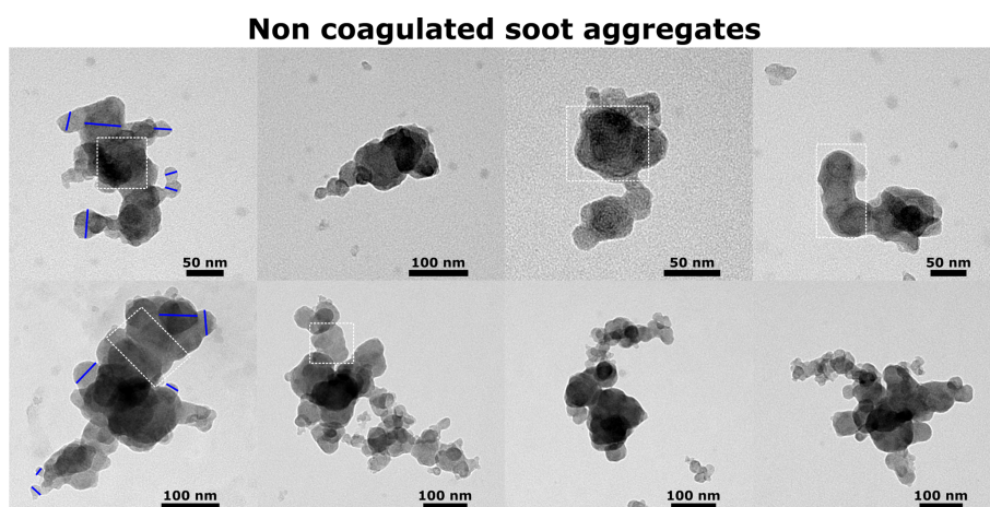
Figure A1. TEM images of soot aggregates collected downstream of the test cell and undergoing no coagulation. The blue lines on two of the images highlight the length of identifiable primary particles. Regions highlighted with dashed white rectangles show fused primary particles. Note the different scale bars in the images.
