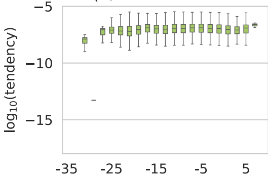
(c) Evap. freezing
