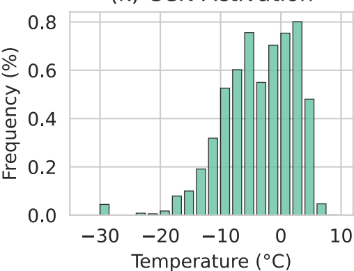
(k) CCN Activation
