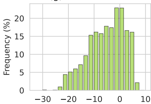
(h) Evap. freezing
