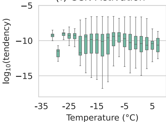
(f) CCN Activation
