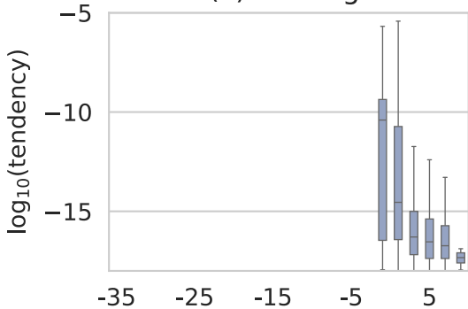
(e) Hom/Het nucl.
