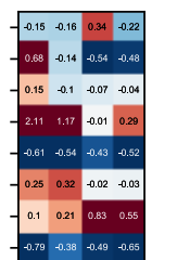
MLC-CHEM (0.1)
