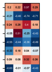
CMAQ M3Dry-psn (0.12)
