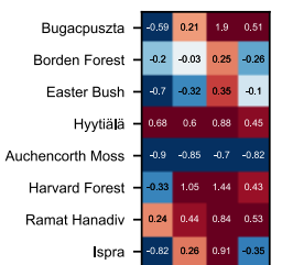
WRF-Chem Wesely (0.17)
