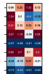
CMAQ M3Dry (0.14)
