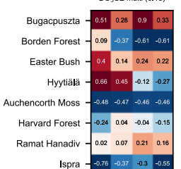
DO 3 SE multi (0.13)
