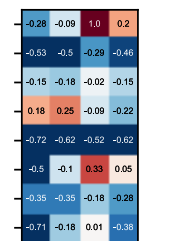
TEMIR Wesely Medlyn (0.18)
