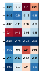
TEMIR Zhang (0.15)
