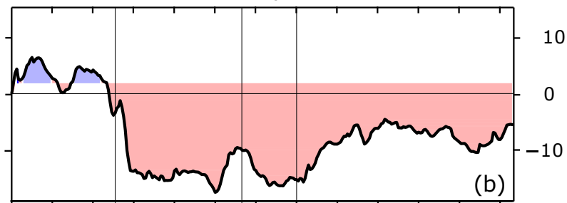
ACLOUD: May/June 2017
