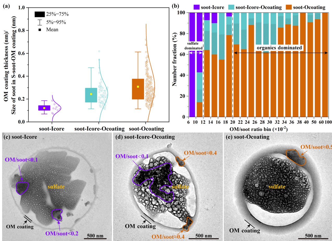
Figure 8. Variations in the OM / soot ratios with different distribution positions of soot in S-soot-OM coating particles. (a) The different ratios of OM / soot in the S-soot-OM coating particles. (b) Number fractions of soot-I-core, soot-I-core-O-coating, and soot-O-coating particles in all S-soot-OM coating particles in different ratios of OM / soot. The oblique bar represents the distribution of soot within the OM coating in all of the soot-I-core-O-coating particles. (c) A typical TEM image of a soot-I-core particle with two soot particles in a sulfate core (OM / soot < 0.2). (d) A typical TEM image of a soot-I-core-O-coating particle with a soot particle in a sulfate core (OM / soot < 0.1) and two soot particles in an OM coating (OM / soot \approx 0.4). (e) A typical TEM image of a soot-O-coating particle with a soot particle in the OM coating (OM / soot \approx 0.5).
