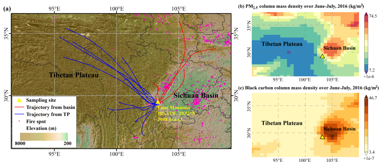
Figure 1. Location of the sampling site, with 24 h backward trajectories during 22 June–9 July 2016, and PM 2.5 and BC column mass density covering the eastern TP and Sichuan Basin in June–July 2016. (a) Location of the sampling site, with the Sichuan Basin on the eastern side and the TP on the western side (29.52° N, 103.33° E; 3048 m a.s.l. – above sea level). The 24 h backward trajectories of each individual particle sample collection time were calculated using the Hybrid Single-Particle Lagrangian Integrated Trajectory model (HYSPLIT). Blue lines represent the western TP trajectories, and red lines represent the eastern basin trajectories. (b, c) PM 2.5 and BC column mass density covering the eastern TP and Sichuan Basin in June–July 2016 (NASA Giovanni online data system; https://giovanni.gsfc.nasa.gov/giovanni/ , last access: 1 July 2023).
