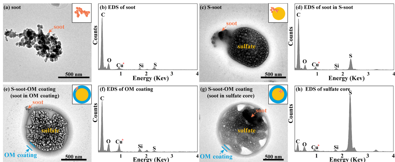
Figure 2. The major types of soot-containing particles in this study. (a) A TEM image of soot. (b) EDS spectrum of soot. The asterisk represents Cu, which was excluded from the EDS detection due to the copper material of TEM grids. (c) A TEM image of S-soot. (d) EDS spectrum of soot in S-soot. (e) A TEM image of the S-soot-OM coating with soot in the OM coating. (f) EDS spectrum of OM coating. (g) A TEM image of the S-soot-OM coating with soot in the sulfate core. (h) EDS spectrum of the sulfate core. All conceptual graphs are placed in the top-right corner of each image. The orange circle aggregates, yellow circles, and blue rings represent soot, sulfate, and OM coatings, respectively.
