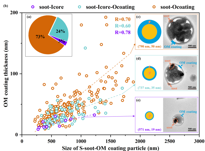
Figure 6. (a) The proportions of soot-Icore, soot-Icore-Ocoating, and soot-Ocoating particles in all S-soot-OM coating particles. (b) The scatter distribution of the particle sizes and OM coating thicknesses of the analysed S-soot-OM coating particles. Conceptual graphs and TEM images of (c) a soot-Ocoating particle, (d) a soot-Icore-Ocoating particle, and (e) a soot-Icore particle. The first and second number in each set of parentheses represents the average size and OM coating thickness of the corresponding S-soot-OM coating particle, respectively.
