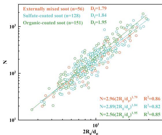
Figure 10. Fractal dimension ( D_f ) of externally mixed soot, sulfate-coated soot, and organic-coated soot on Mount Emei. The parameter n in parenthesis represents the total number of soot particles analysed for each soot category to calculate D_f .
