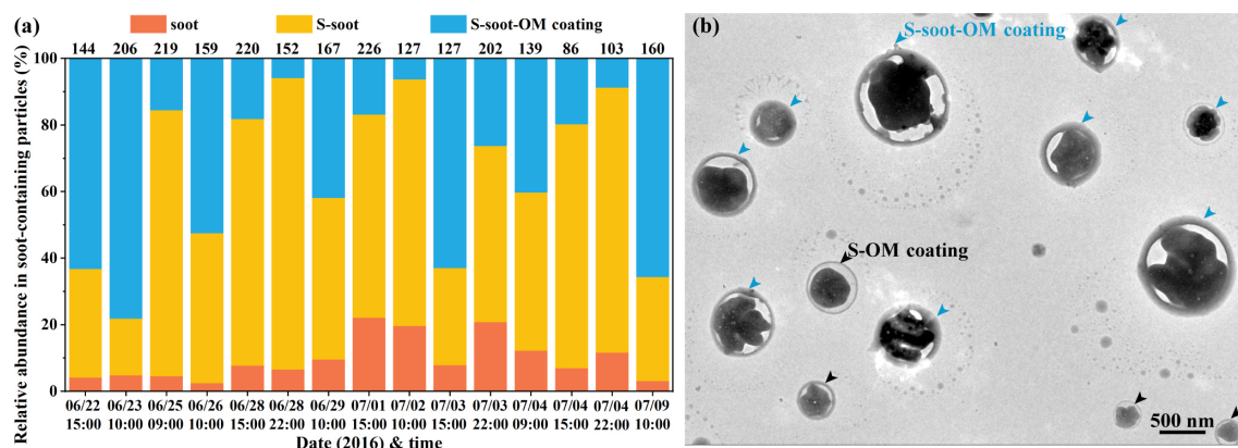
Figure 4. (a) Relative abundance of soot, S-soot, and S-soot-OM coating particles in all soot-containing particles at the Mount Emei site at each sampling time from 22 June to 9 July 2016. A total of 2437 soot-containing particles were analysed, and the number of analysed particles is shown above the column. (b) A typical TEM image with abundant S-soot-OM coating particles in the sample at 10:00 LT on 23 June.
