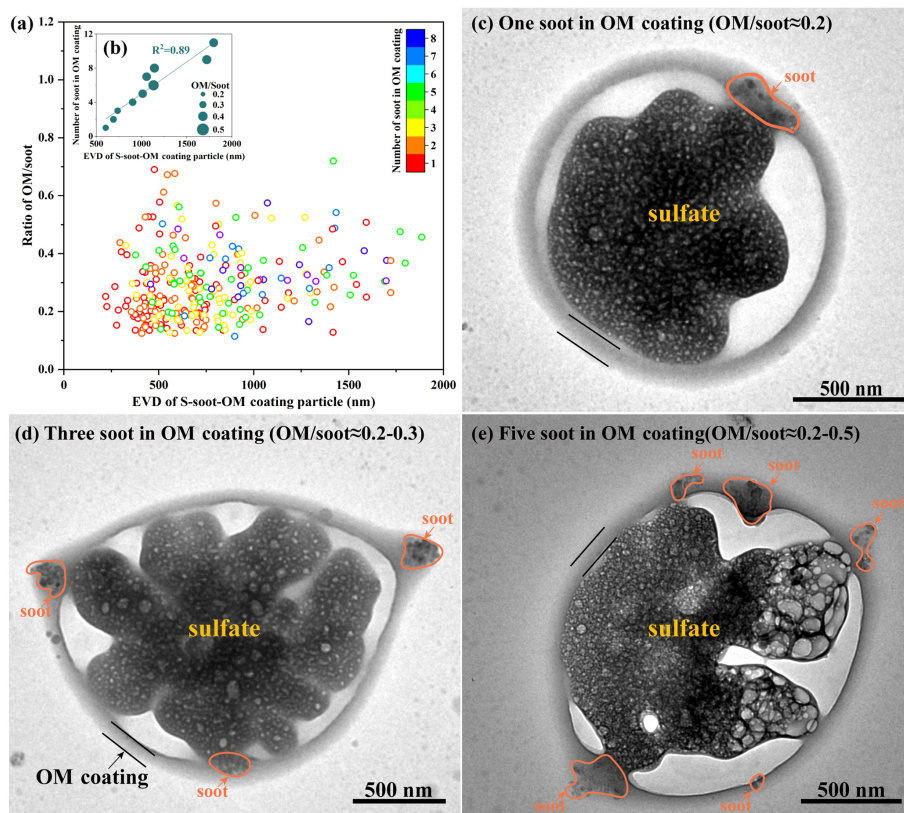
Figure 9. (a) Scatter diagram of OM / soot and the particle size of the S–soot–OM coating particles. Different colours represent the number of soot particles being captured in the OM coating. (b) Correlation between the average size of the S–soot–OM coating particle and the average number of soot particles in the OM coating. The size of the circle point represents the average ratio of OM / soot. (c) A typical TEM image of a S–soot–OM coating particle with one soot particle in an OM coating (OM / soot \approx 0.2; the size of S–soot–OM coating is \approx 336 nm). (d) A typical TEM image of a S–soot–OM coating particle with three soot particles in an OM coating (OM / soot \approx 0.2–0.3; the size of S–soot–OM coating is \approx 652 nm). (e) A typical TEM image of a S–soot–OM coating particle with five soot particles in an OM coating (OM / soot \approx 0.2–0.5; the size of S–soot–OM coating is \approx 582 nm).
