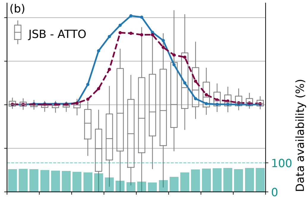
Latent heat flux
