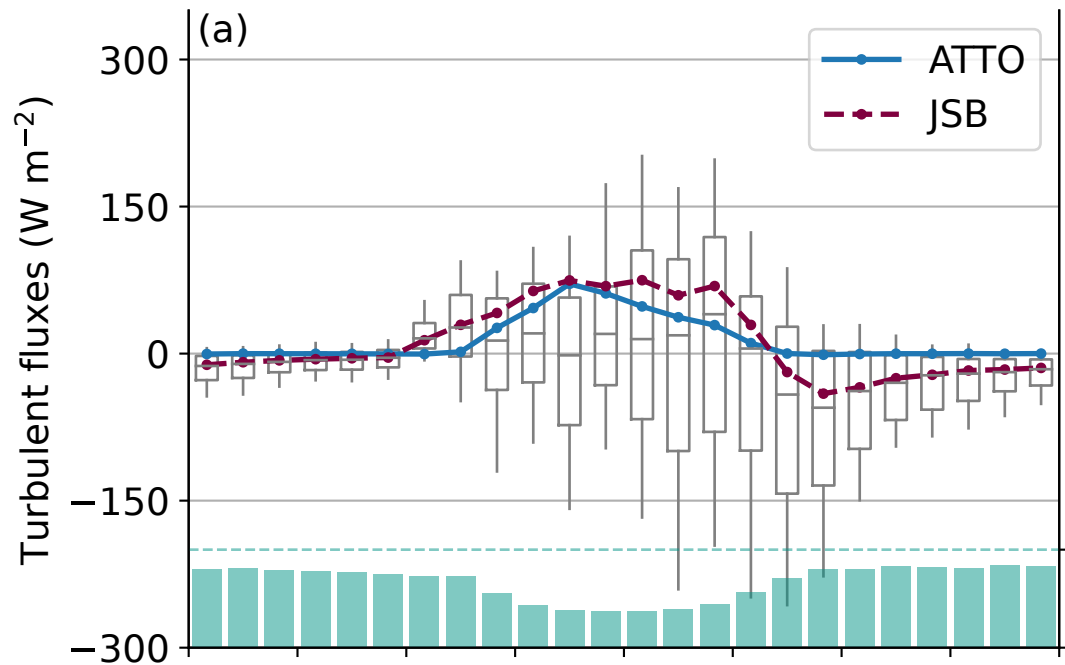
Sensible heat flux
