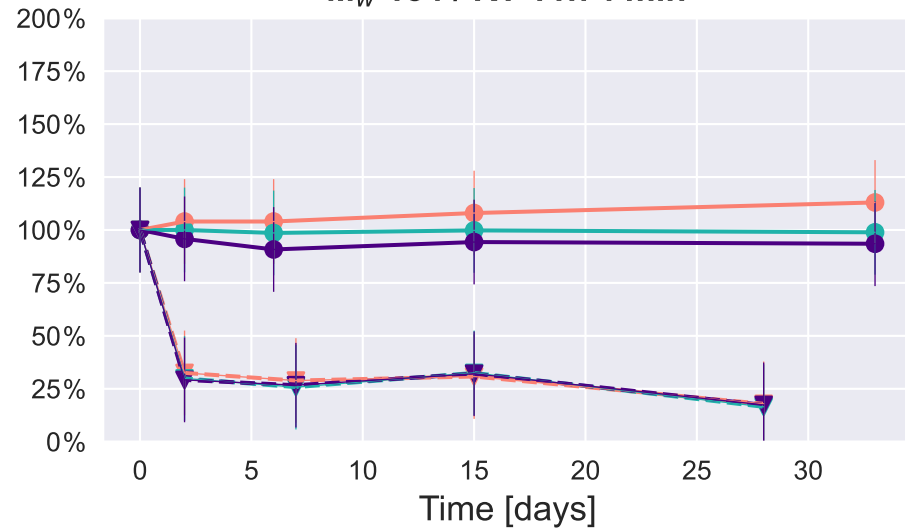
M w 184 / RT 11.74 min
