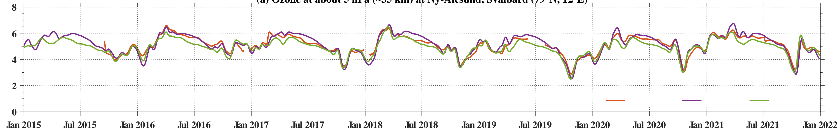
(b) Ozone at about 5 hPa (~35 km) at Conjugate latitude station (79° S, 12° E)
