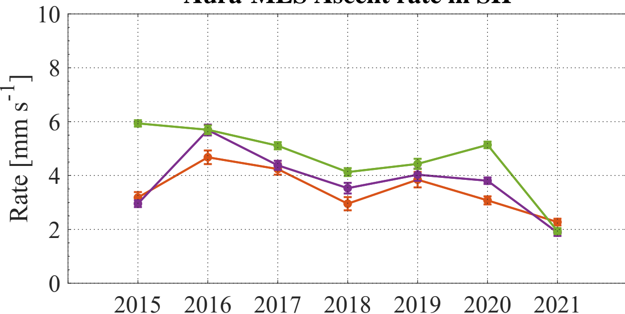
Aura-MLS Ascent rate in SH
