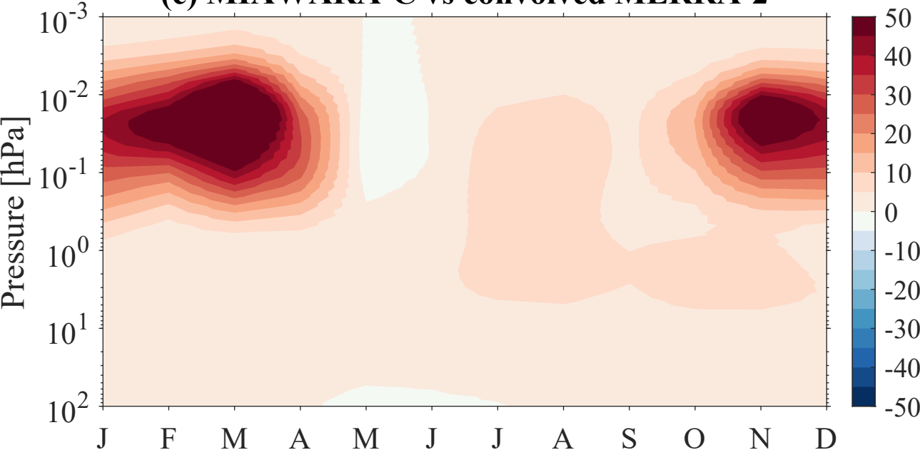
(c) MIAWARA-C vs convolved MERRA-2
