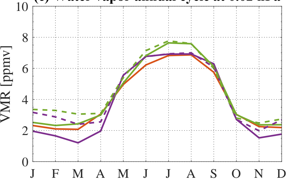
(c) Water vapor annual cycle at 0.02 hPa
