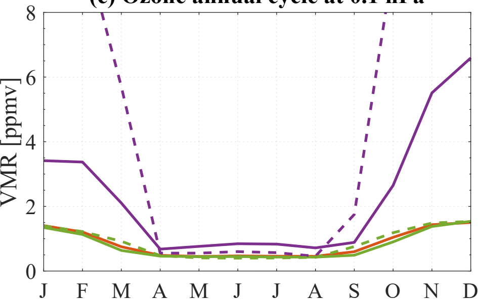
(c) Ozone annual cycle at 0.1 hPa
