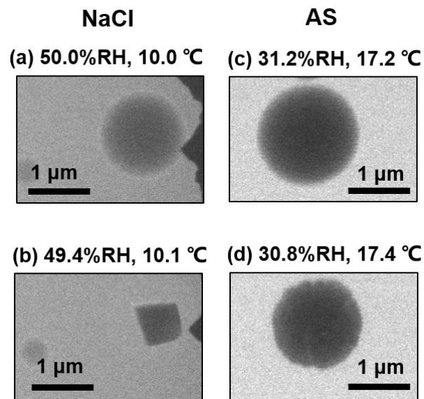
Figure S2 ESEM images of efflorescence processes for (a–b) NaCl and (c–d) AS particles.
