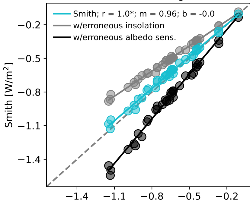
(c) SW ERF ari (absorption)
