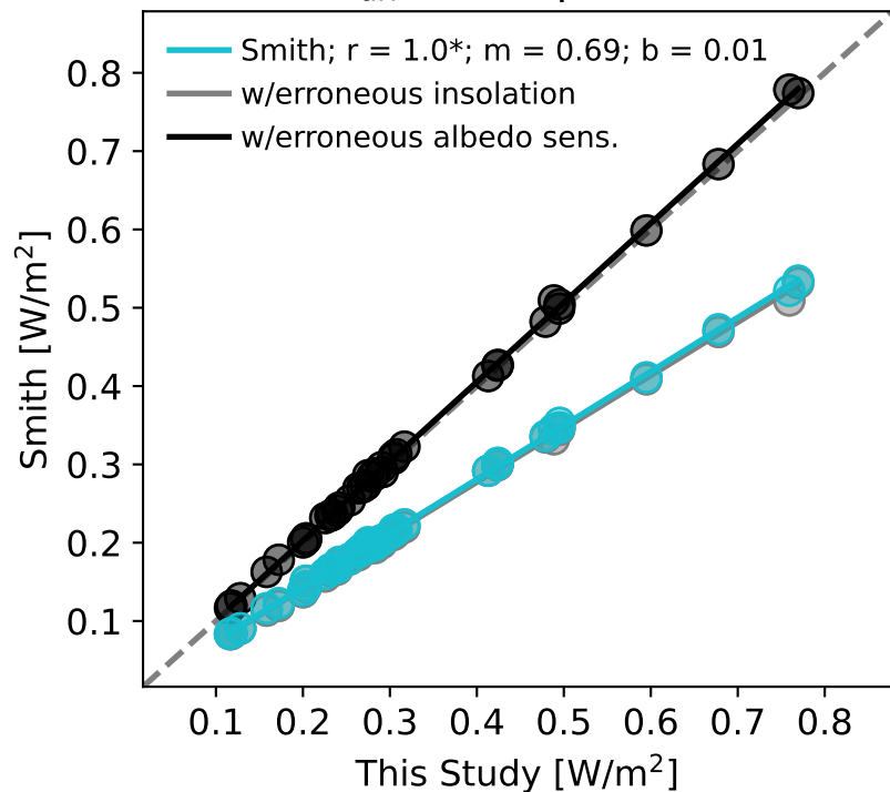
(c) SW ERF ari (absorption)
