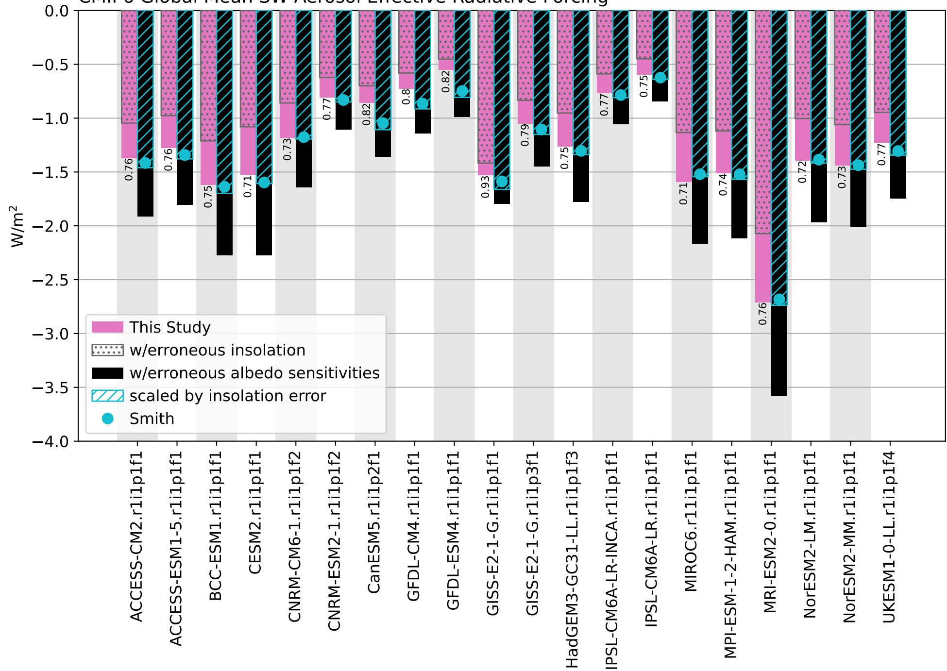
CMIP6 Global Mean SW Aerosol Effective Radiative Forcing
