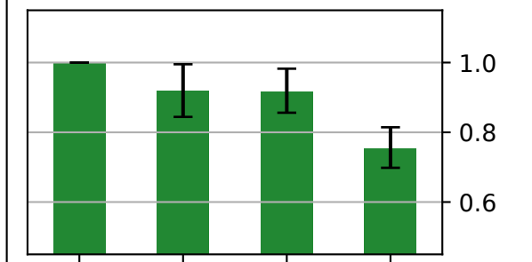
(e) Cluster 4
