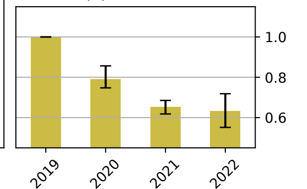
(e) Cluster 4
