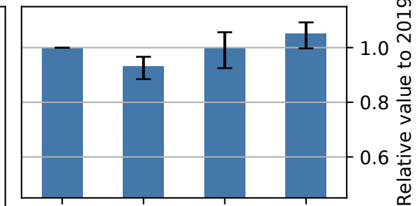
(c) Cluster 2
