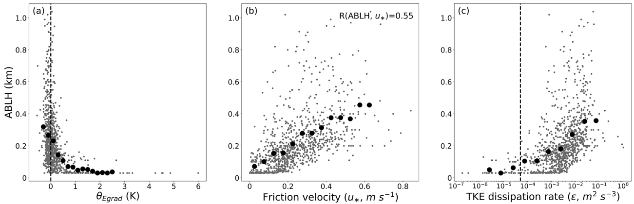
Figure 11. The ABLHs and bin-averaged values for (a) equivalent potential temperature gradient, \theta_{\text{Egrad}} (K); (b) friction velocity, u_* ( \text{m s}^{-1} ); and (c) turbulent kinetic energy dissipation rate, \varepsilon ( \text{m}^2 \text{s}^{-3} ). The average bins for \theta_{\text{Egrad}} , u_* , and \varepsilon logarithm are 0.2 K, 0.05 \text{ m s}^{-1} , and 0.5 \text{ m}^2 \text{ s}^{-3} , respectively. The correlation coefficient R is given in panel (b), which shows statistically significant results ( p < 0.05 ). The dashed vertical lines indicate the thresholds of (a) \theta_{\text{Egrad}} = 0 \text{ K} and (c) \varepsilon = 5 \times 10^{-5} \text{ m}^2 \text{ s}^{-3} .
