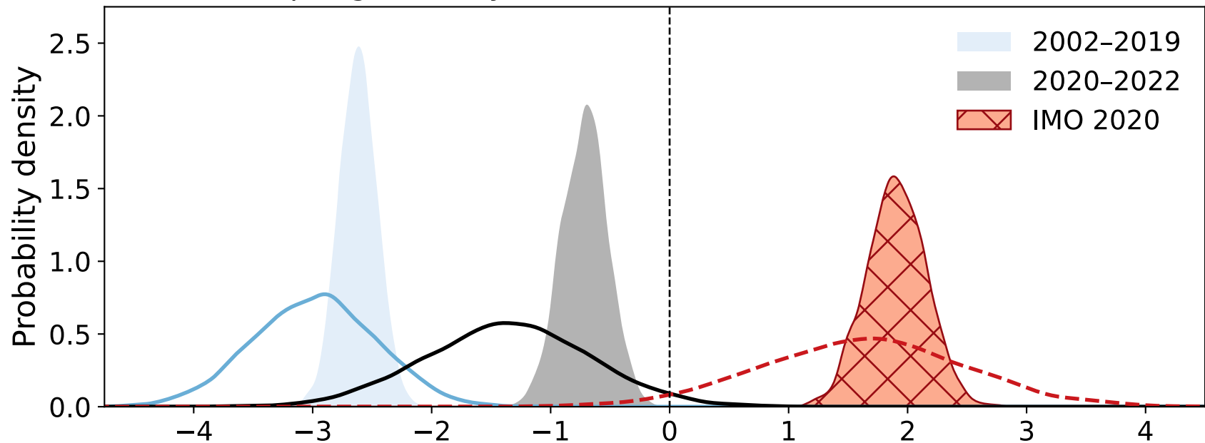
(a) Austral spring Twomey effect estimates ( \text{W m}^{-2} )
