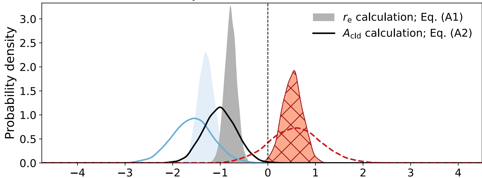
(b) Annual mean Twomey effect estimates ( \text{W m}^{-2} )
