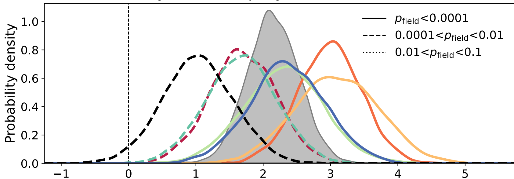
(c) Relative change in annual mean r_e (%)
