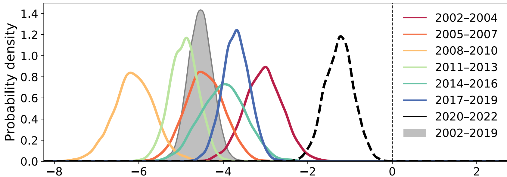
(b) Relative change in austral spring A_{\text{cld}} (%)
