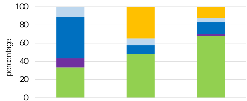
(b) O 3 UNECE SOURCES SUMMER 2010
