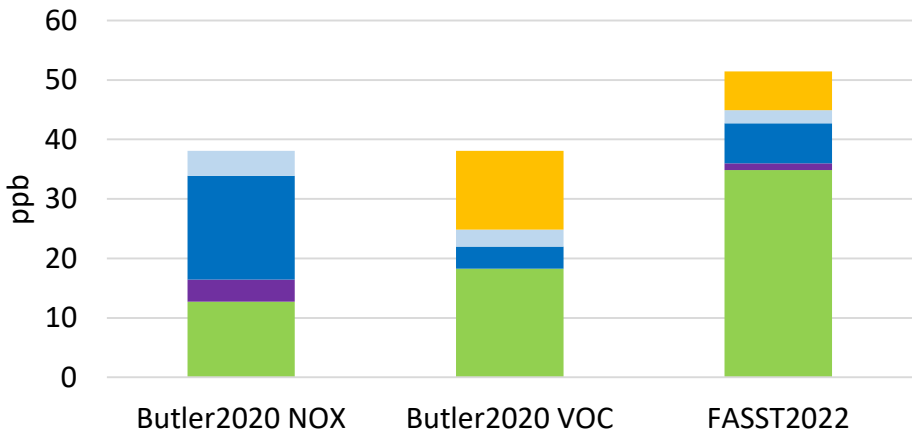
(a) O 3 UNECE SOURCES SUMMMER 2010
