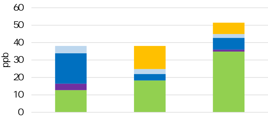
(a) O 3 UNECE SOURCES SUMMER 2010
