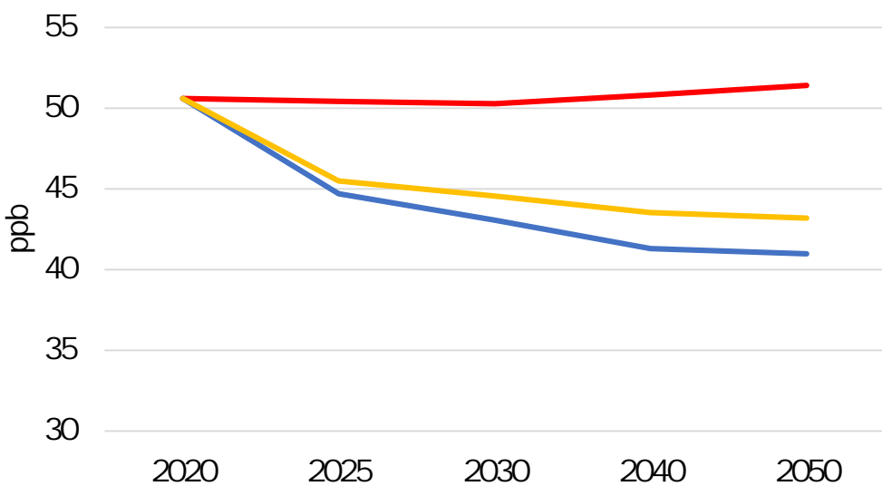
O 3 exposure metric
