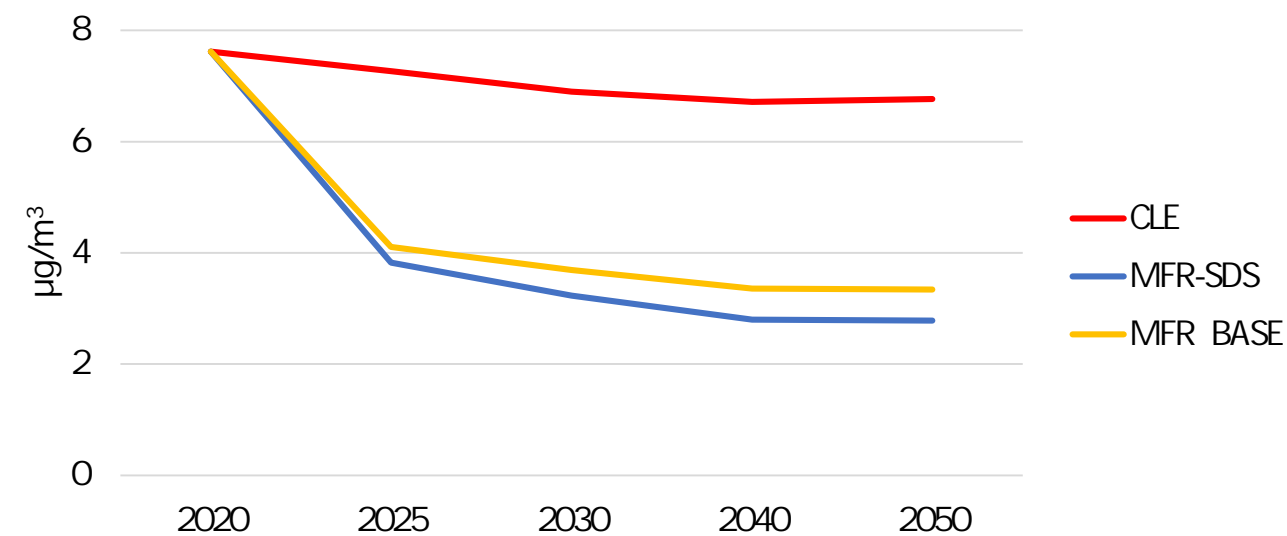
PM 2.5 exposure metric
