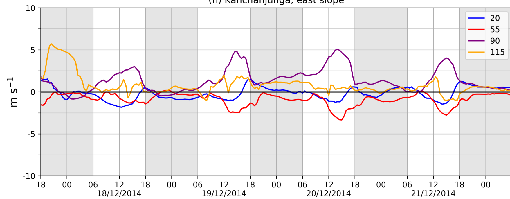
(h) Kanchanjunga, east slope
