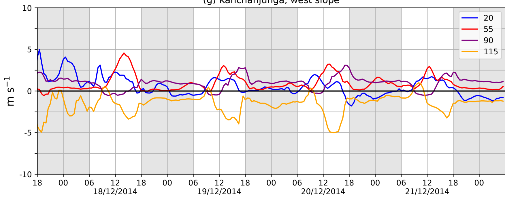
(g) Kanchanjunga, west slope
