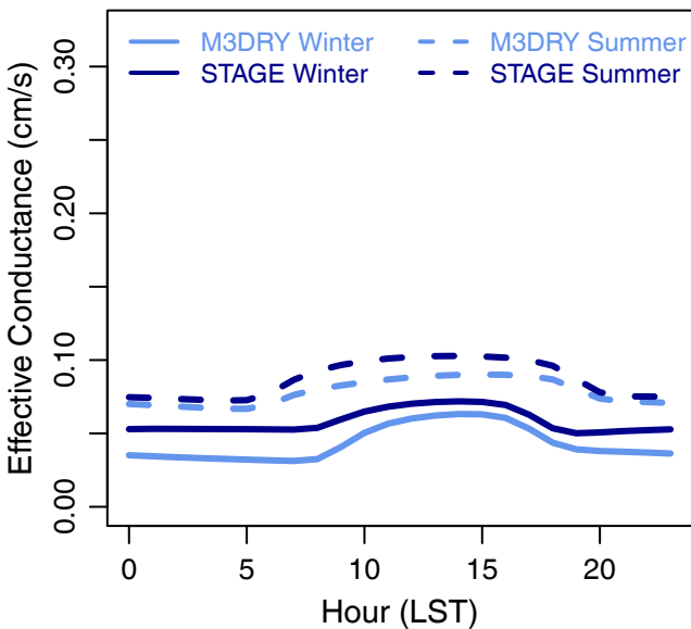
Cuticular Effective Conductance O_3
