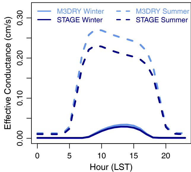
Stomatal Effective Conductance O_3
