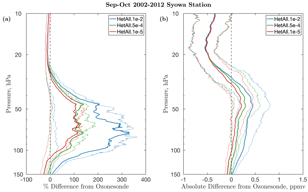
Figure S4. Same as Fig. 7 b and c for ozone of the main manuscript, but showing Syowa Station without the noHetAll simulation.
