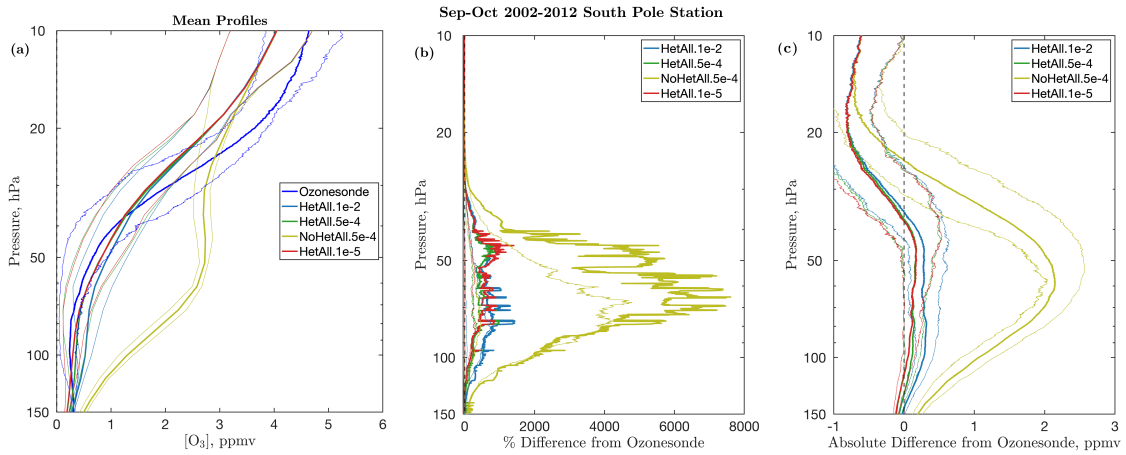
Figure S5. Same as Fig. 7 a to c for ozone of the main manuscript, but showing South Pole Station.
