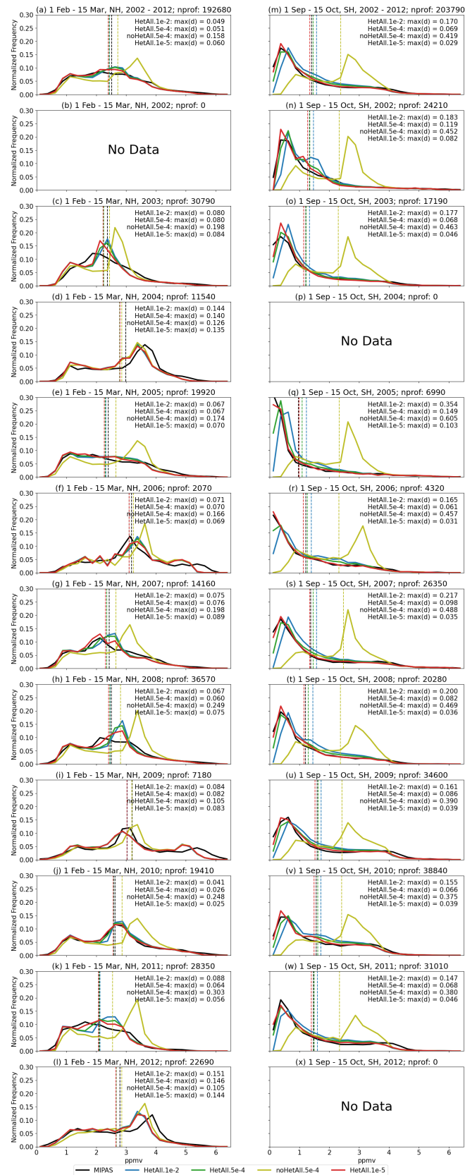
Figure S3. Same as Fig. 6 ( O_3 ) of the main manuscript, but showing all individual years.
