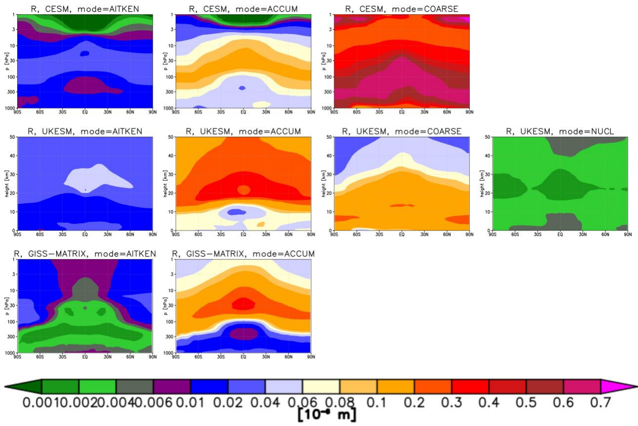
Figure S1: Mean radius in each mode for all models in the Equatorial injection case.
