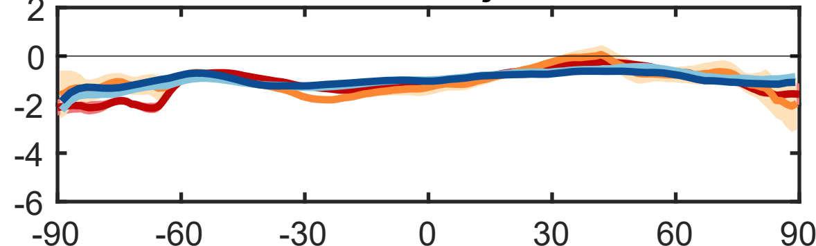
Normalized \Delta T_s - Injection at 30°S
