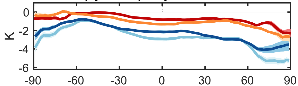
(7y mean) - Injection at 15°S
