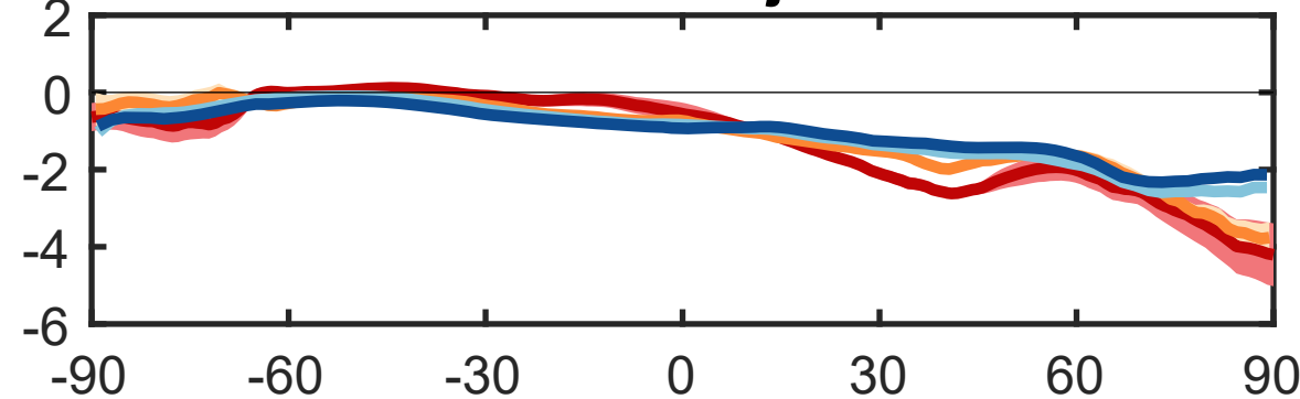
Normalized \Delta T_s - Injection at 0°N
