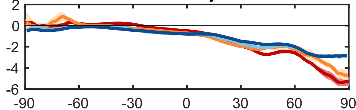
Normalized \Delta T_s - Injection at 15°N
