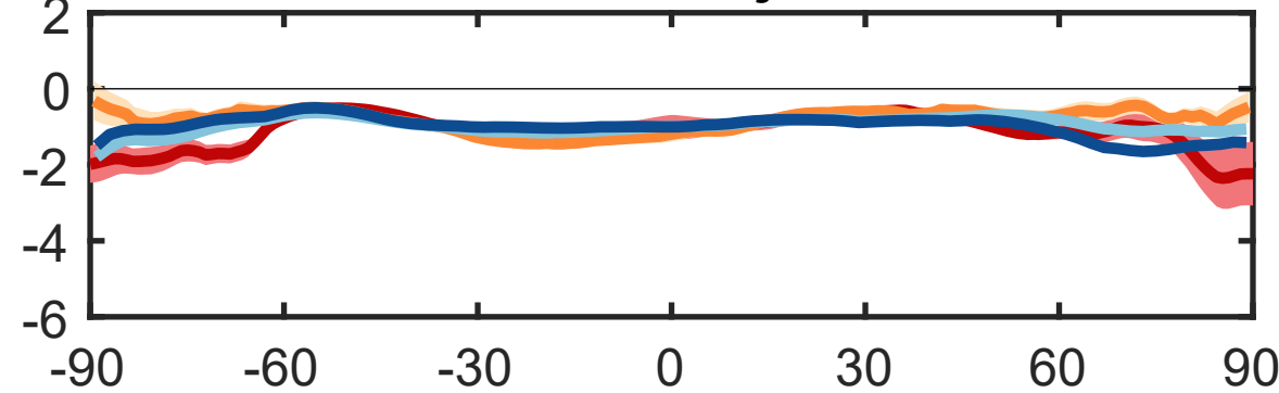
Normalized \Delta T_s - Injection at 30°S
