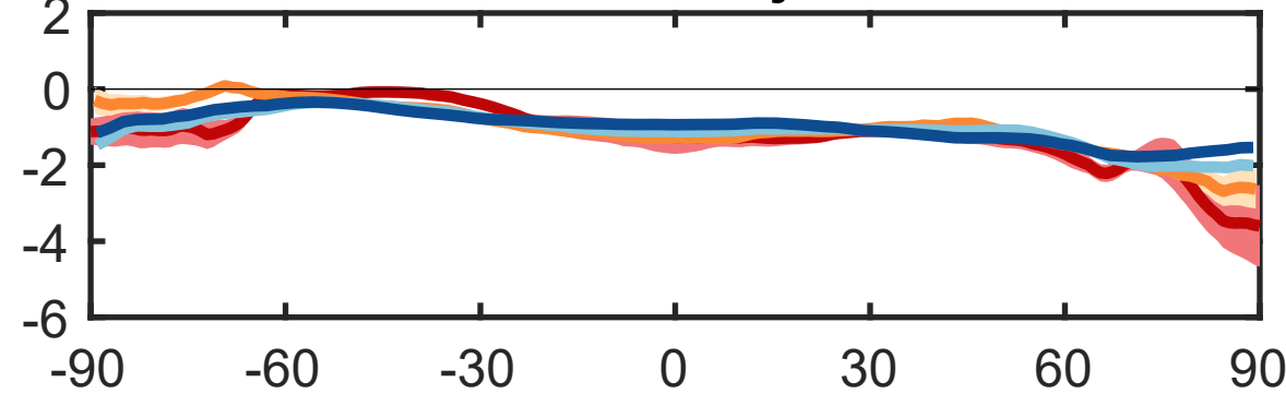
Normalized \Delta T_s - Injection at 15°S
