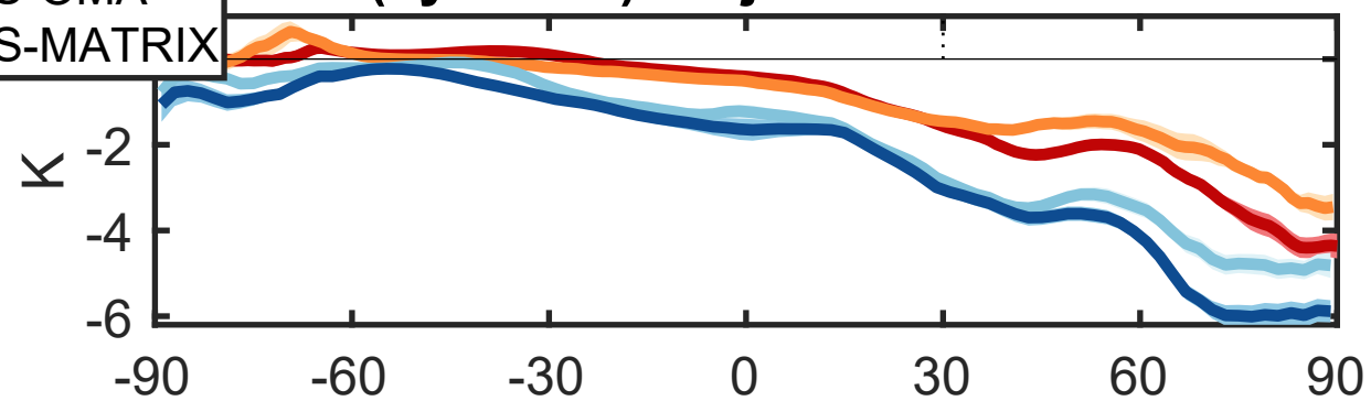
(7y mean) - Injection at 15°N
