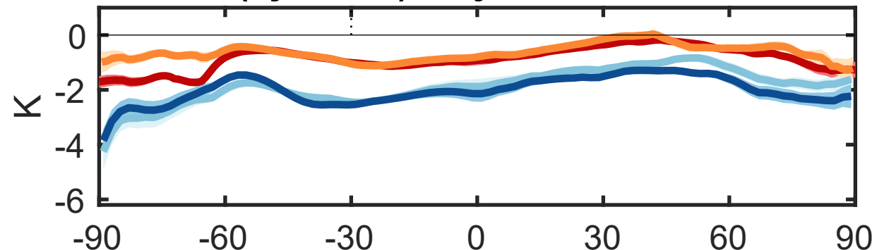
(7y mean) - Injection at 30°S
