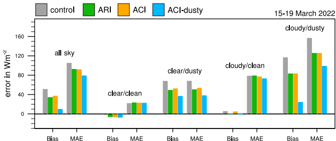
(c) downward shortwave radiation at the surface
