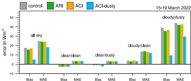
(c) downward shortwave radiation at the surface
