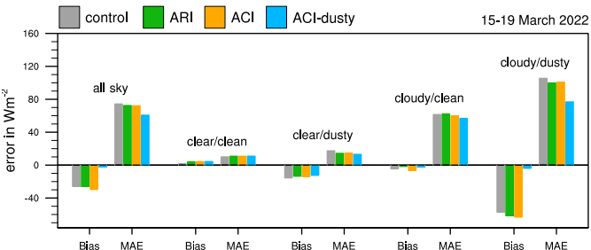
(b) reflected shortwave radiation at TOA
