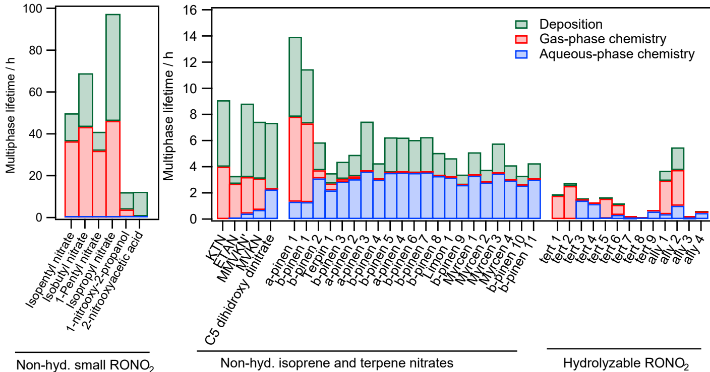
(b) Wet aerosol conditons (LWC = 3 x 10 -5 g m -3 )
