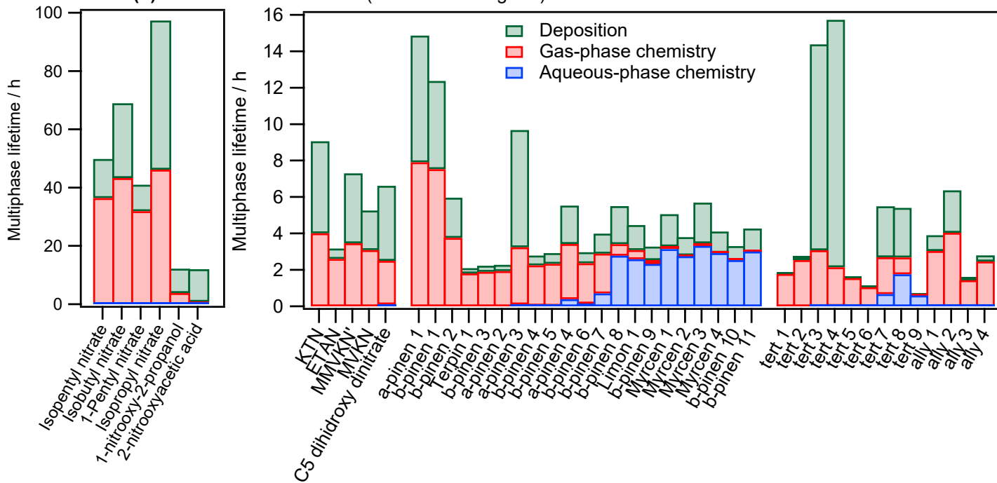
(b) Wet aerosol conditons (LWC = 3 x 10 -5 g m -3 )
