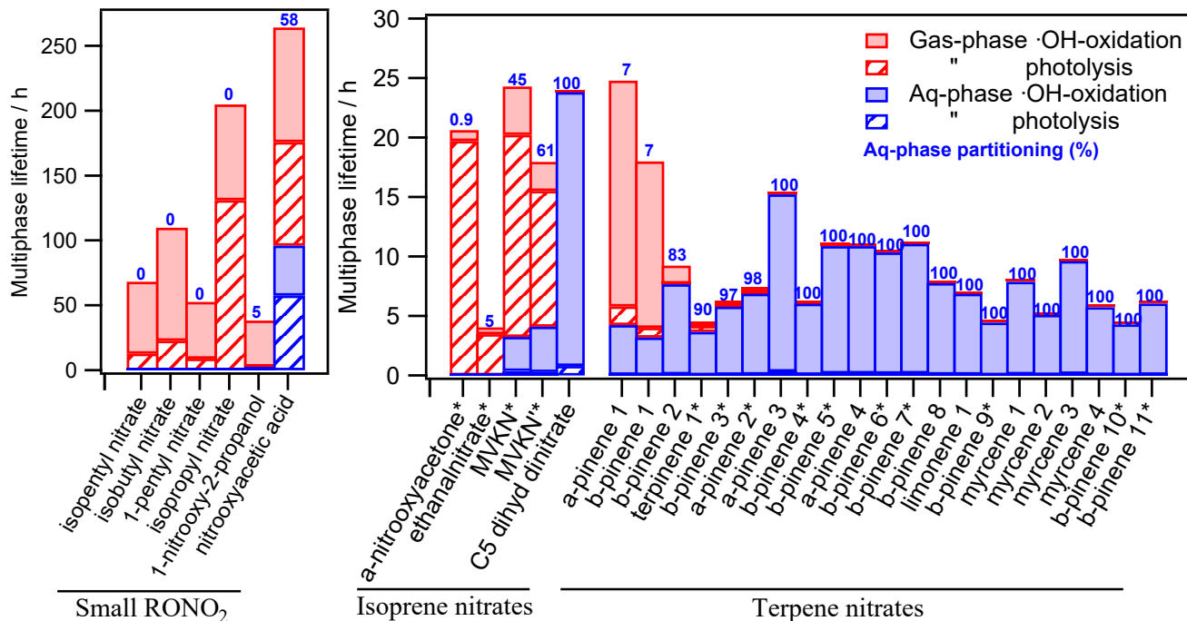
(b) Wet aerosol conditions ( LWC = 3 \times 10^{-5} \text{ g m}^{-3} )
