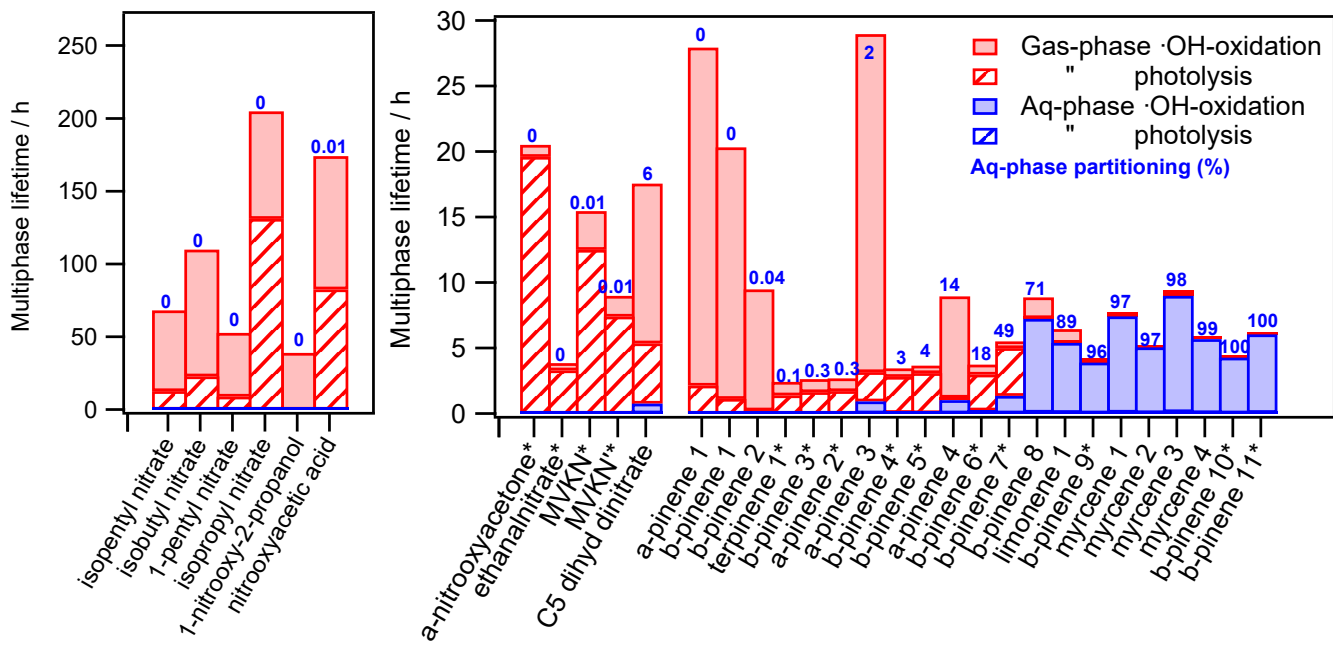
(b) Wet aerosol conditions ( LWC = 3 \times 10^{-5} \text{ g m}^{-3} )
