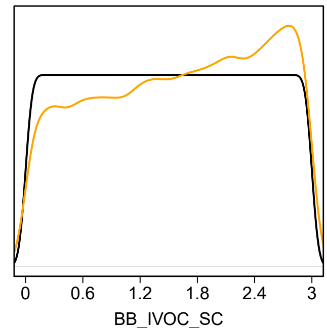
9. BB_IVOC_SC
