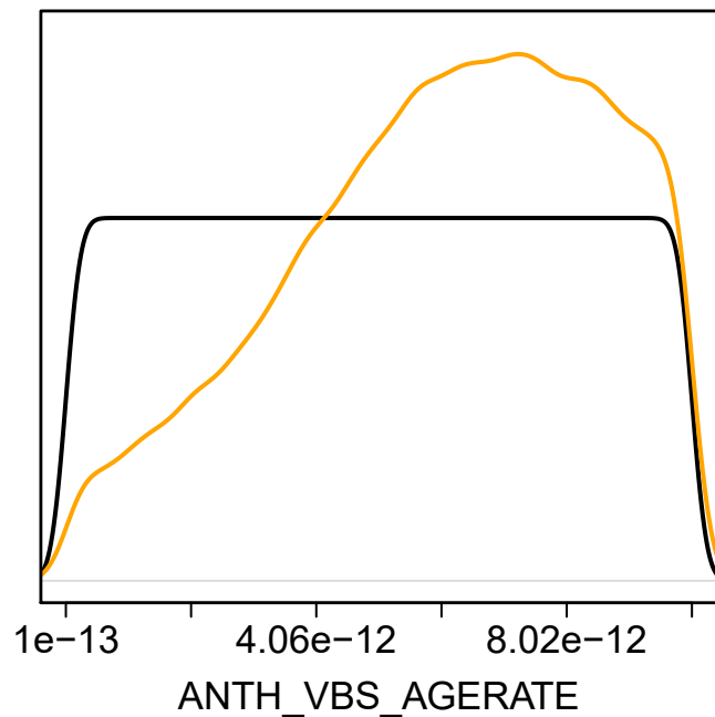
1. ANTH_VBS_AGERATE
