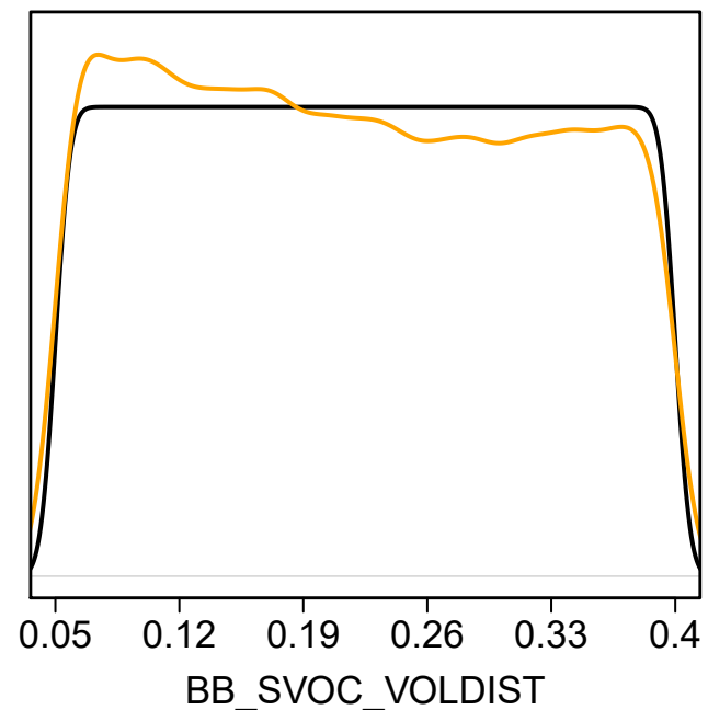
7. BB_SVOC_VOLDIST
