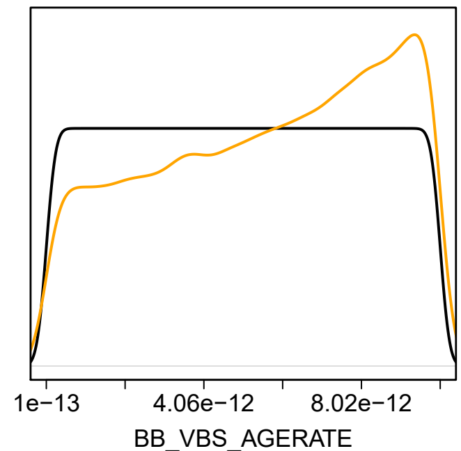
6. BB_VBS_AGERATE
