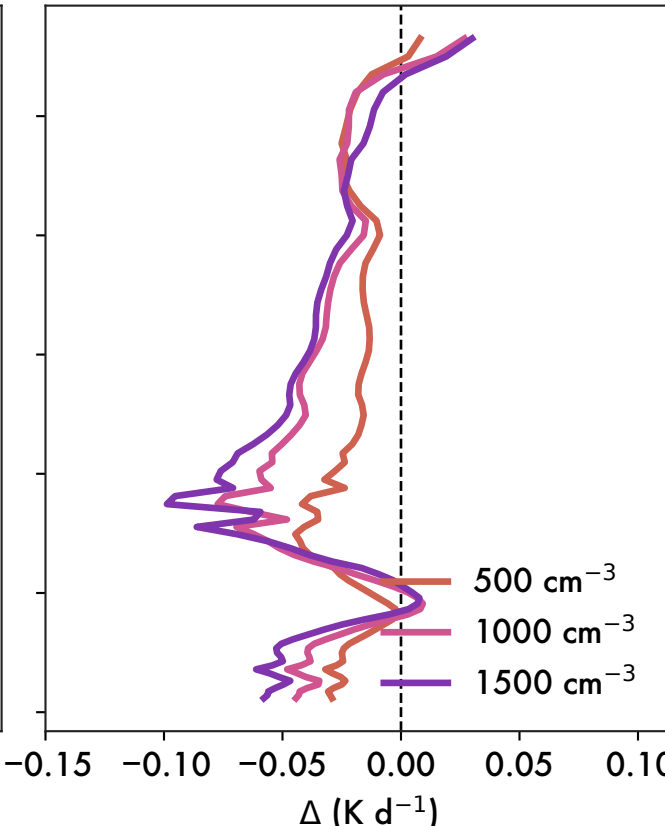
(b) \Delta Ammonium Sulfate
