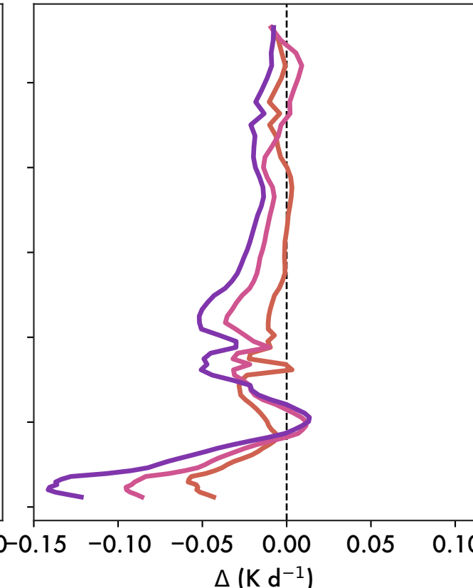
(c) \Delta Sea Salt
