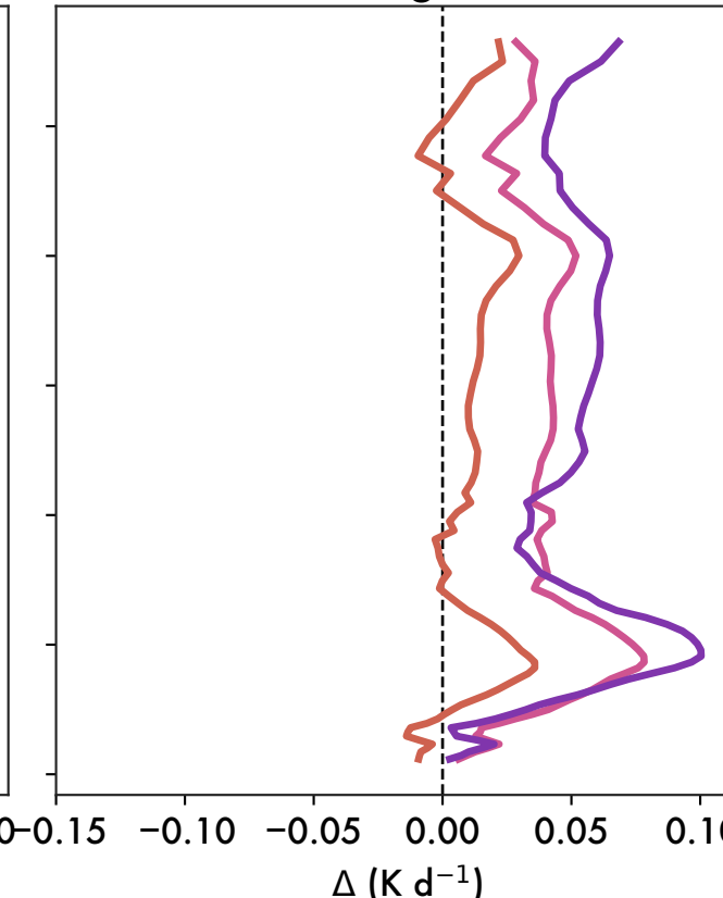
(e) \Delta Absorbing Carbon
