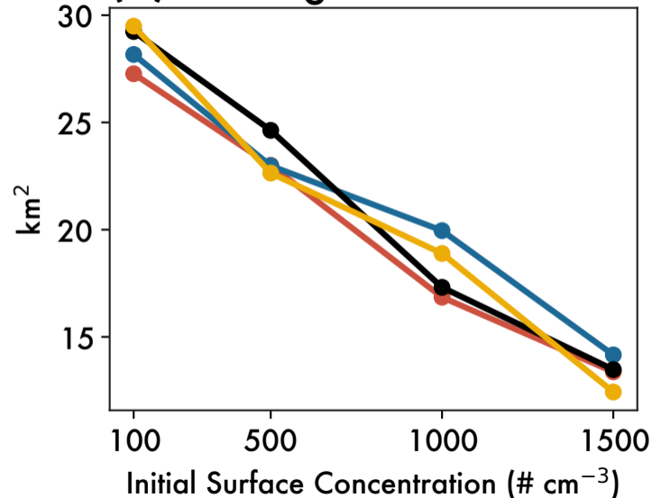
(b) Raining Area
