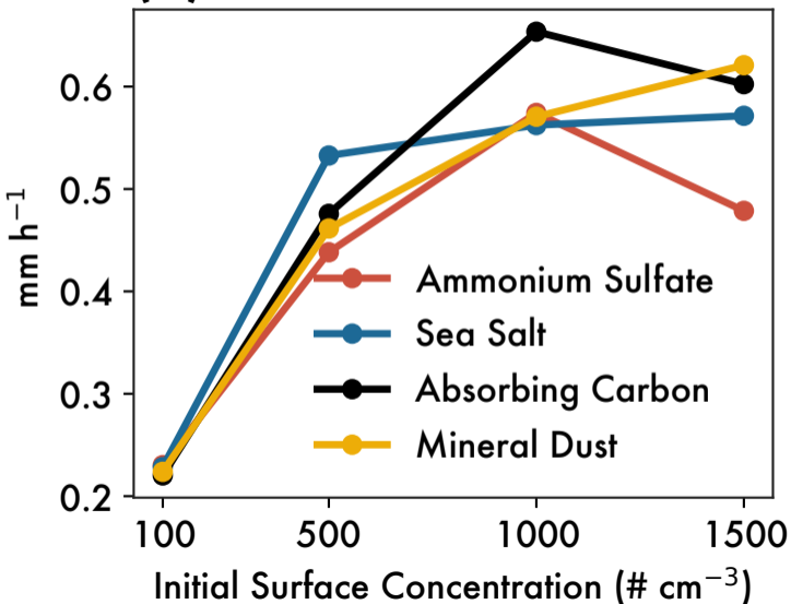
(a) Rain Rate
