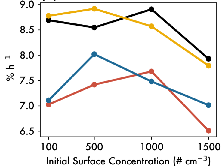
(c) Norm. Aero. Rainout Rate
