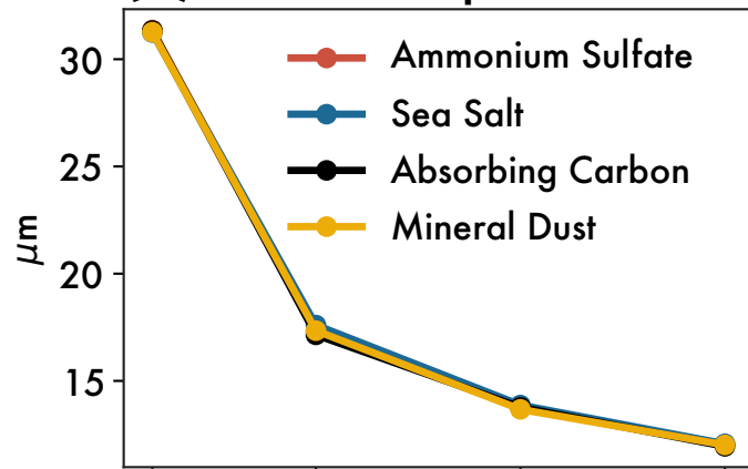
(b) Cloud Drop Diameter
