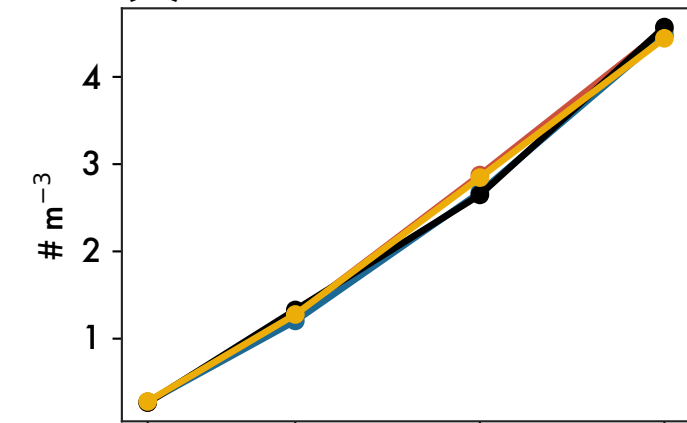
(a) Cloud Number Conc.
