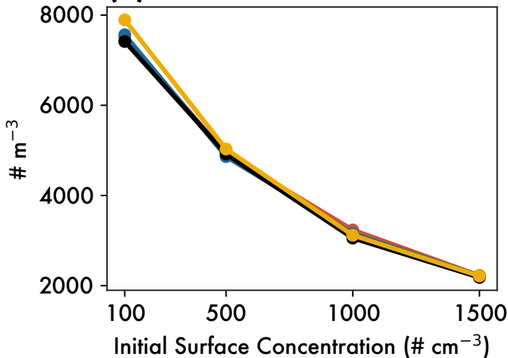
(c) Rain Number Conc.
